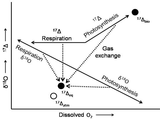
Figure 5. A schematic diagram showing the effects of photosynthesis, respiration and air-water gas exchange on dissolved O 2 concentrations, δ 18 O and 17 Δ. δ 18 O changes with all the processes and additionally is also affected by mixing. Because of non-mass dependent processes occurring in the stratosphere, the 17 Δ of O 2 in air has a different signal to the O 2 produced biologically where fractionation is mass-dependent. 17 Δ increases due to photosynthesis, decreases due to gas exchange but is not affected by respiration. Respiration removes O 2 and decreases the dissolved O 2 concentration but fractionates O 2 isotopes in a mass-dependent way, which does not affect the relative proportion of δ 17 O and δ 18 O and therefore the 17 Δ. 17 Δ bio is the maximum value of pure biological signal, which amounts to 17 Δ of water. The slope of 17 Δ increase towards 17 Δ bio is the kinetic slope λ for respiration (λ = 0.518). 17 Δ eq is the O 2 at air-water equilibrium, which has a small offset from 17 Δ atm , which is by definition 0, due to fractionation at equilibrium where δ 17 O and δ 18 O slopes during invasion and evasion follow a slightly different slope to that of respiration.
