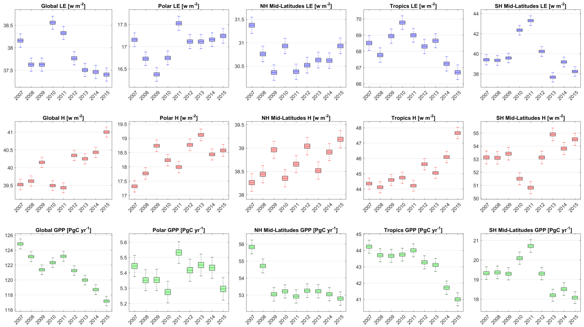
Figure 13: Annual mean estimates and uncertainty bounds of LE (top row), H (middle row) and GPP (bottom row) retrievals at global (left column) and regional (four right columns) scales between 2007 and 2015. The central line in each box indicates the mean, the edges of the box are 25th and 75th percentiles, and the whiskers show the most extreme values.
