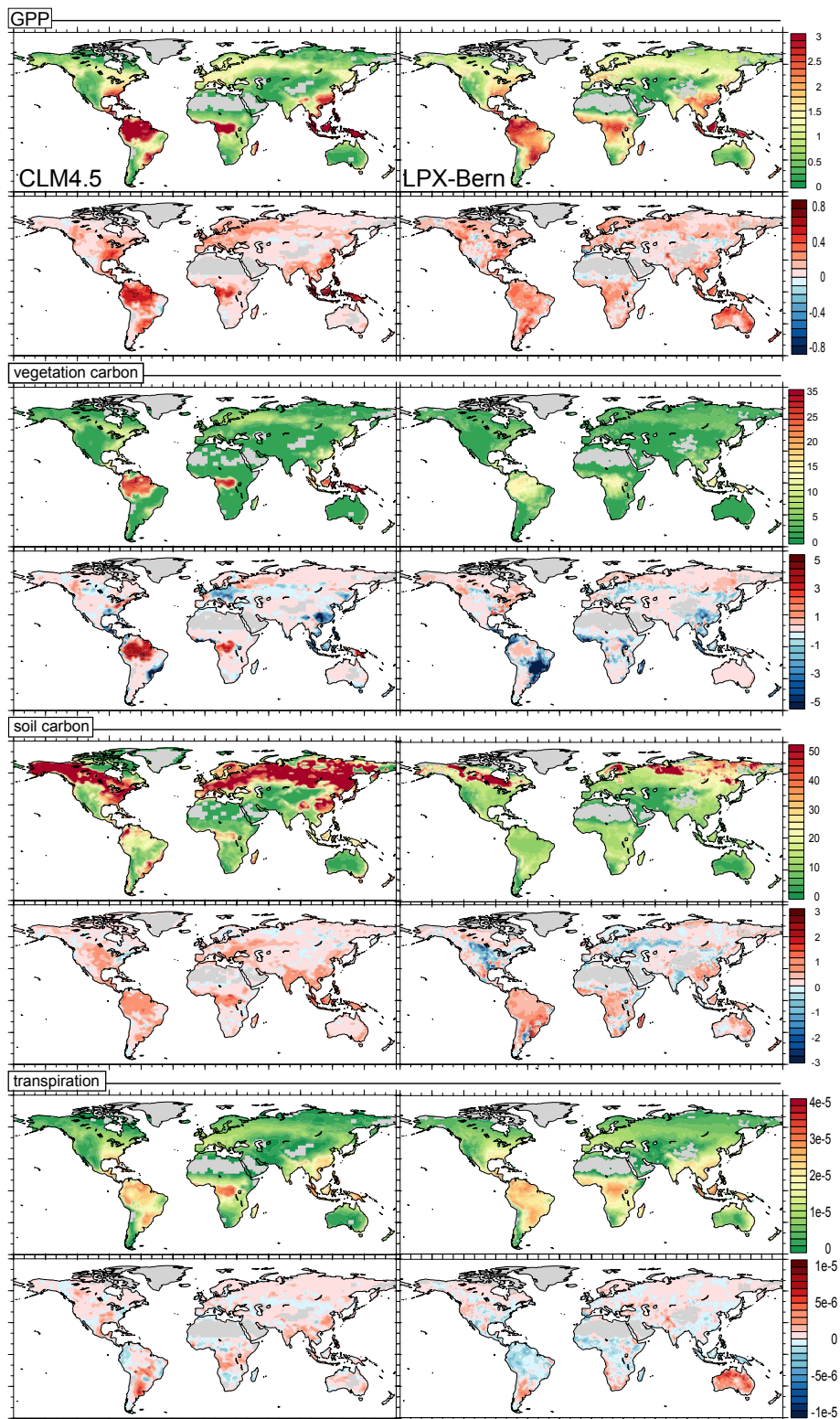
Figure 2. GPP (kgC/m 2 /yr), vegetation carbon (kgC/m 2 ), soil carbon (kgC/m 2 ) and transpiration (mm/s) in the year 2000 (top) and the difference between 1900 and 2000 (below). The estimates are based on 40 decadal means (1996-2005 and 1996-2005 minus 1896-1905, respectively).
