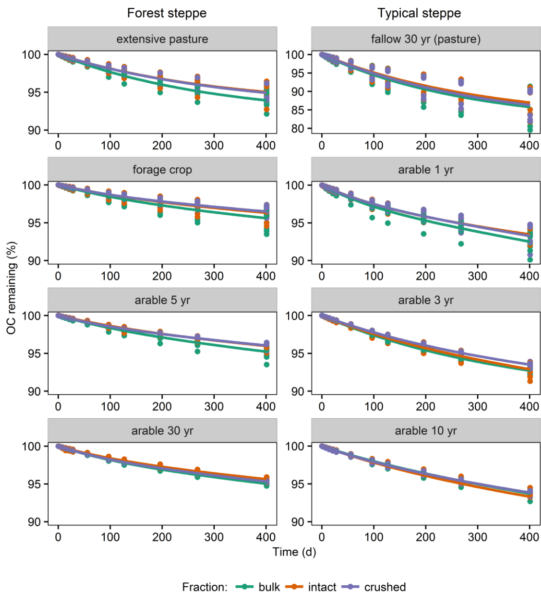
5 Figure 2: Percentage of soil OC remaining in the samples during 401 days of incubation for eight plots within two steppe types and for the three fractions bulk soil, intact macro-aggregates, and crushed macro-aggregates. For all plots a two-pool model (Eq. 2) was fitted, except for the extensively managed plots (extensive pasture and the fallow 30 yr (pasture)), where an asymptotic two-pool model was fitted (Eq. 3). Note the different scale for the fallow 30 yr (pasture).
