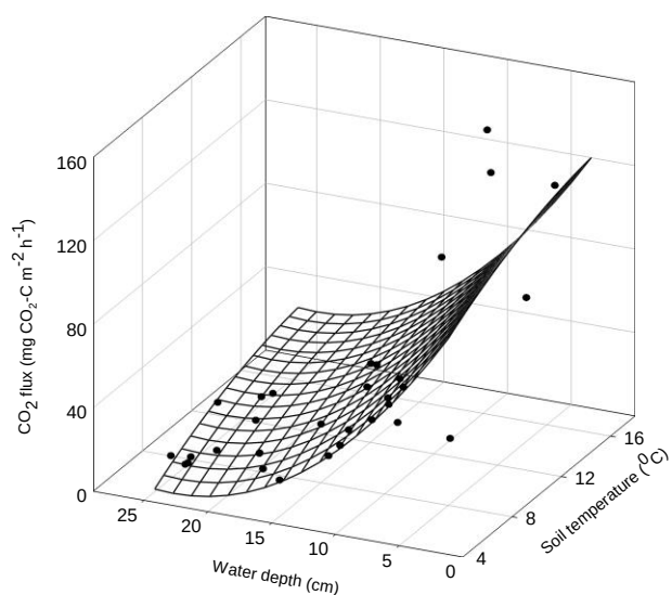
Figure 8. Dependence of CO 2 fluxes on water depth and soil temperature during the intervals in which the LFS is flooded. A significant ( R^2 = 0.62 , P < 0.001 ) 3D Paraboloid regression is shown in the mesh plot. Individual values shown are means (n=3-4).
