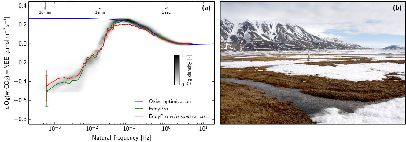
Figure 2. Example of the CO 2 flux estimation during snowmelt. a: Ogive on 31 May 2015, 15:00 LT, showing a mismatch between low and high frequencies. While ogive optimization estimates a net CO 2 release, EddyPro (with and without spectral corrections after Moncrieff et al. (1997, 2004)) indicates an uptake. Average horizontal wind speed was 5.2 m s -1 from NW (313°), air temperature 4.5°C, quality flag 0. Arrows on the top indicate the corresponding time scales. b: Photo of the environment around the flux tower on 27 May 2015, 12:00 LT during snowmelt.
