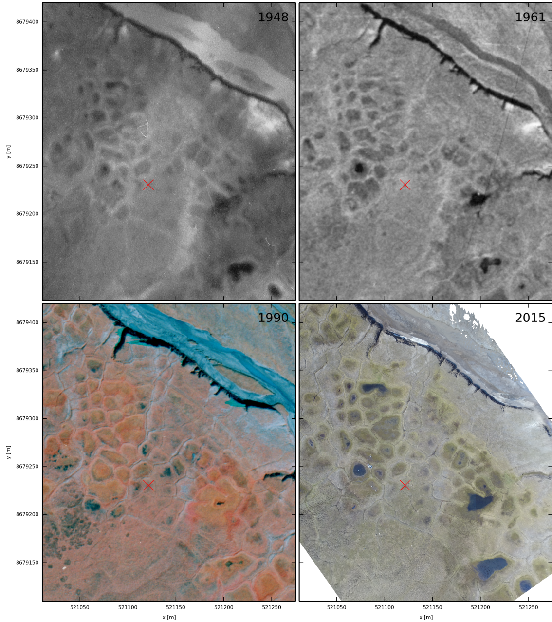
Figure 5. Time series of images of the Adventdalen site showing little signs of differential ground subsidence, which would indicate ice-wedge degradation. The image from 2015 is the same as shown in Fig. 1, while historical photographs were provided by the Norwegian Polar Institute (reference numbers S48-5181, S61-3301 and S90-5273). The images from 1948 and 1961 were taken on panchromatic films, and the image from 1990 is a near infra-red (false color) photography. The red cross marks the EC tower.
