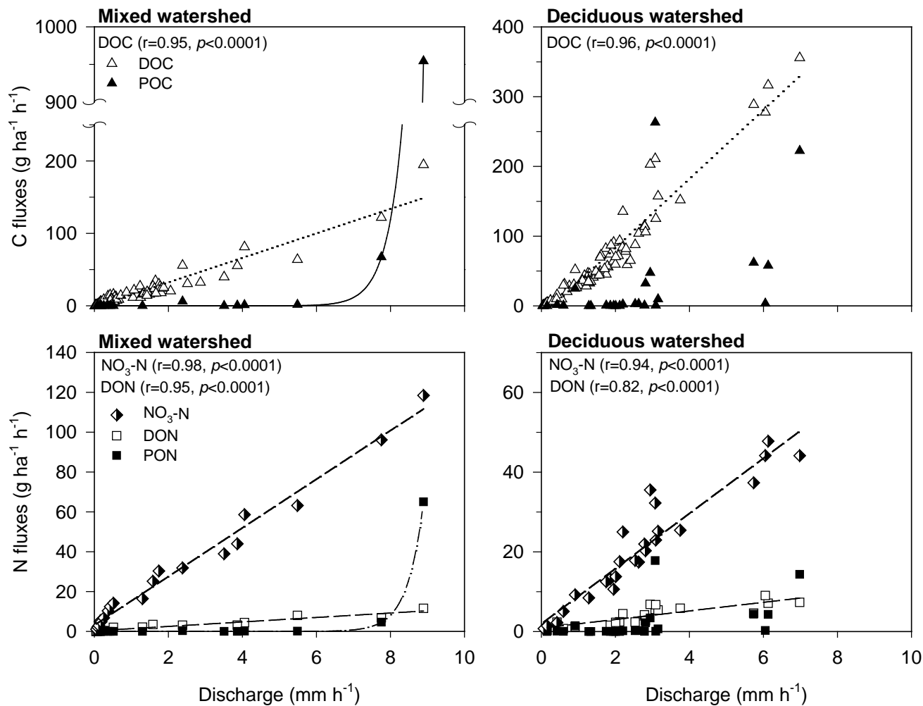
Figure 4: Fluxes of carbon (dissolved organic carbon (DOC) and particulate organic carbon (POC) and nitrogen (dissolved organic nitrogen (DON), and particulate organic nitrogen (PON) and nitrate (NO 3 -N) in runoff with discharge during monsoon storm events.
