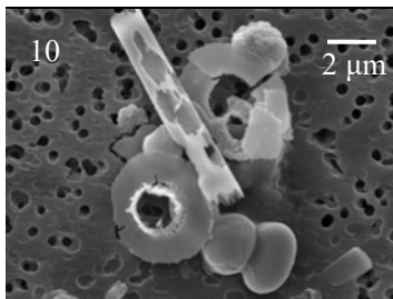
U. sp. 1 coccolith detached
