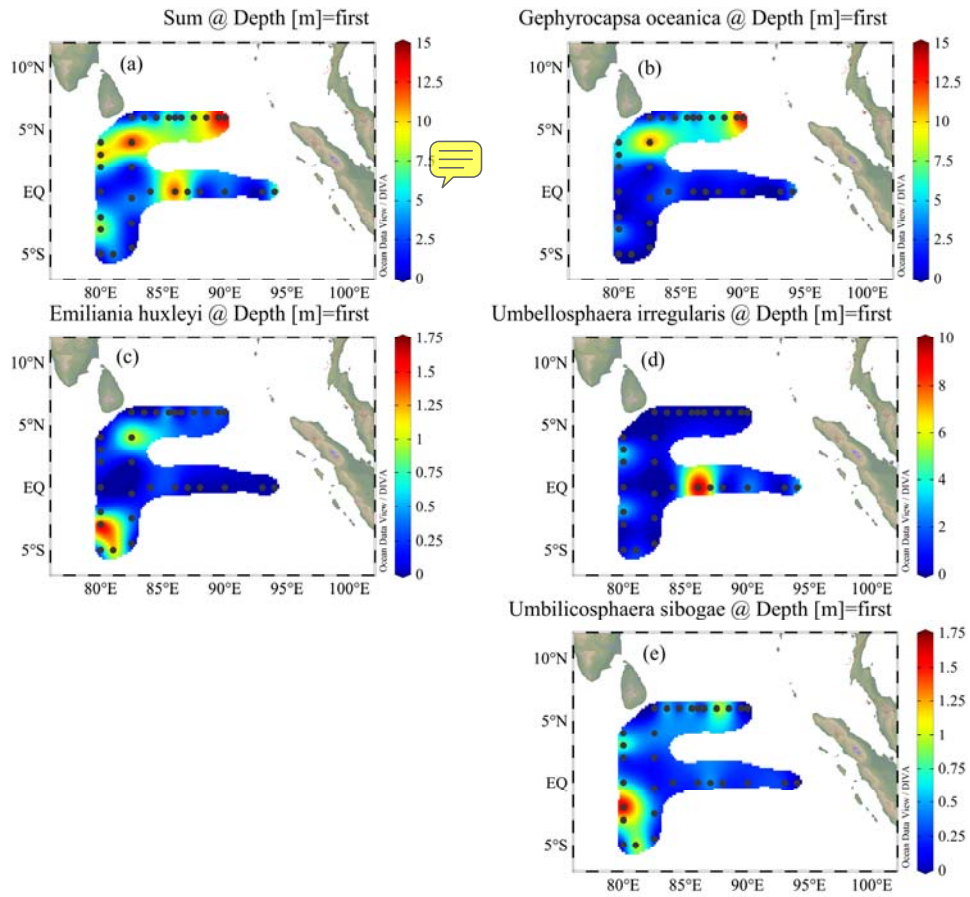
Fig. 5. The surface distribution of dominant coccospheres (units: cells l^{-1} ) in the surveyed area.
