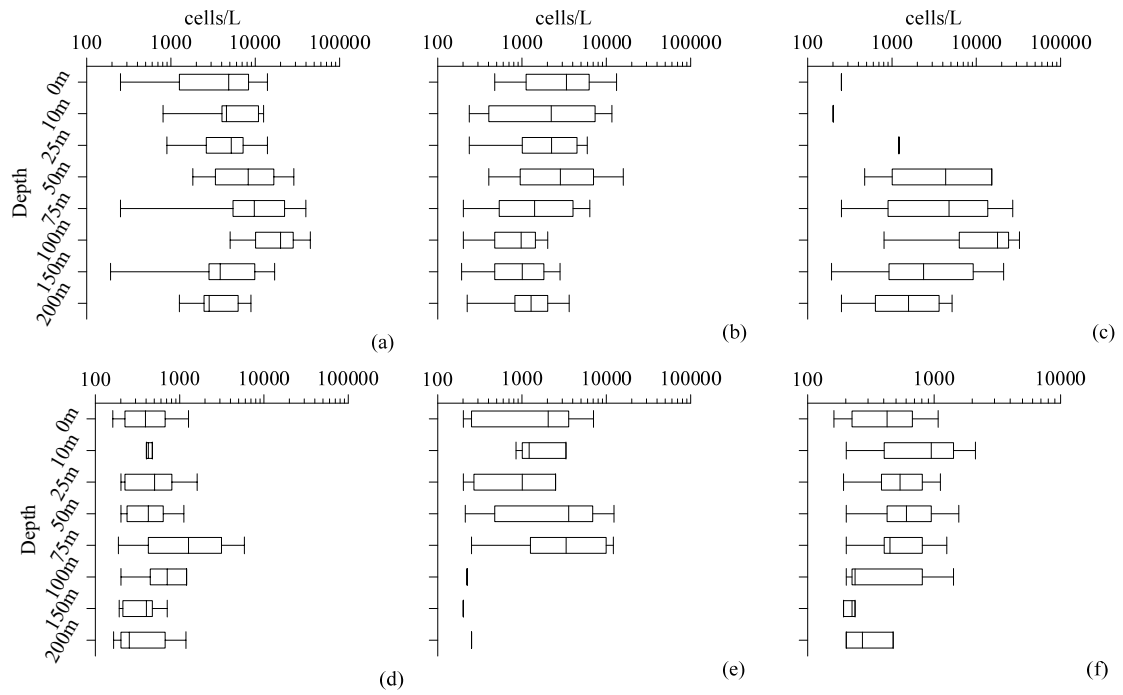
Fig. 11. Vertical distributions of dominant coccospheres (units: cells l -1 ) in the surveyed area. (a) Sum; (b) Gephyrocapsa oceanica ; (c) Florisphaera profunda ; (d) Emiliana huxleyi ; (e) Umbellosphaera irregularis ; (f) Umbilicosphaera sibogae
