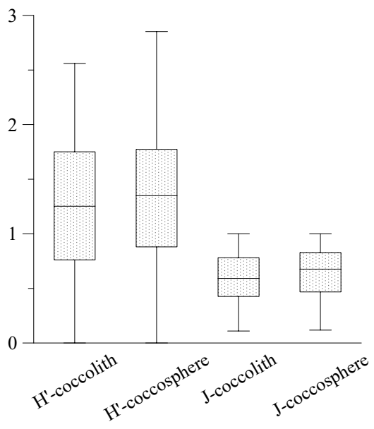
Fig. 16. Box and whisker diagrams of biodiversity index of coccolithophore in the surveyed area.
