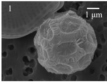
E. huxleyi type A overcalcified
