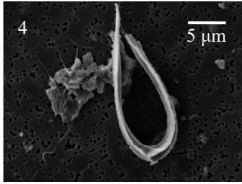
C. cristatus CER telesmus type
