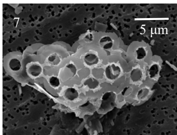
U. sp. 1 cell collapsed
