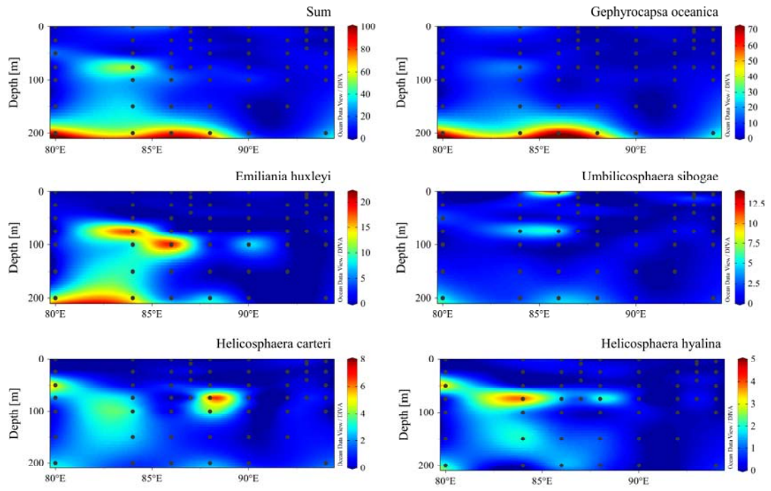
Fig. 6. Dominant coccolith distributions (units: coccoliths l -1 ) along section A of the surveyed area.
