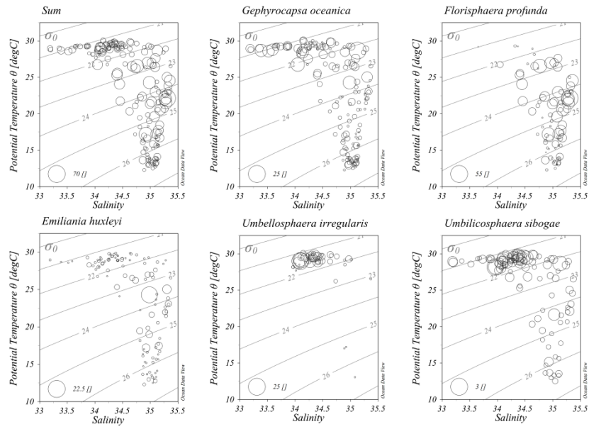
Fig. 18. Scatter plots of coccophere distribution under T-S properties in the surveyed area.
