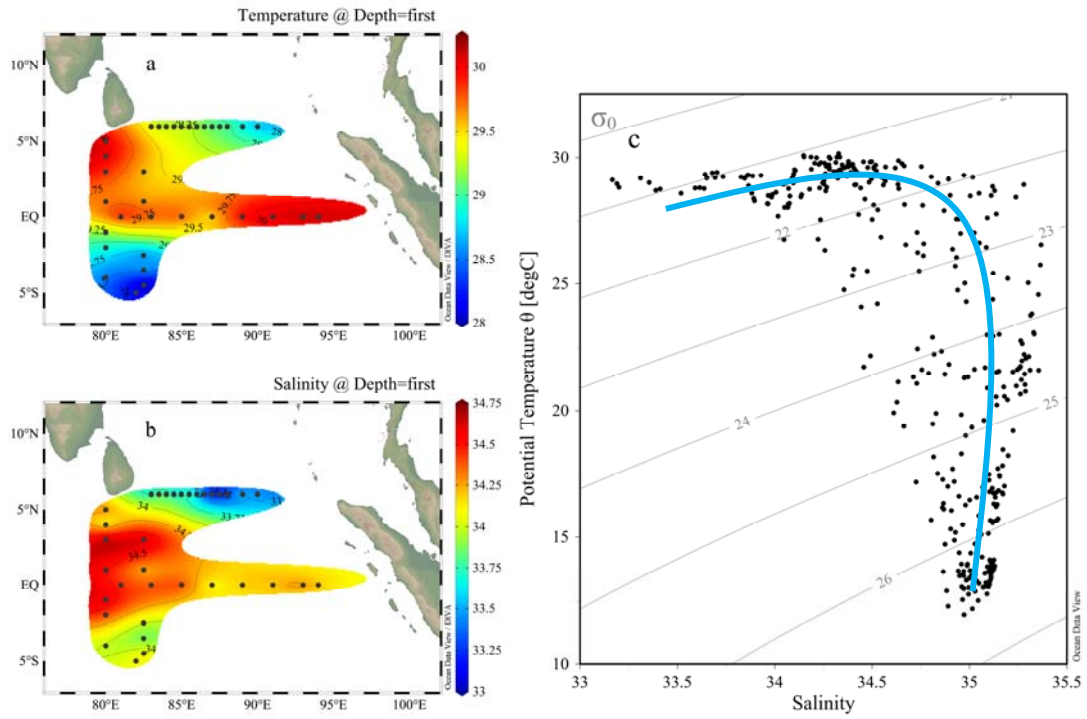
Fig. 2. Sea surface temperature ( ^{\circ}\text{C} ) and salinity in the surveyed area (left); Temperature-salinity (T-S) diagram in the surveyed area, the blue solid line shows an the inversed-L-shape of the hydrologic data (right).
