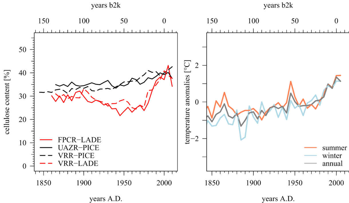
5 Fig. 4. Modern cellulose content chronologies per site and species (left) and temperature anomalies shown for the NW and SW subregions within the Greater Alpine Region from HISTALP for summer (April-September) and winter (October-March) half-year and per year (right). The CC [%] chronologies are calculated as arithmetic means from individual series for their common period (sample replication \geq 4 ). HISTALP data is given for summer season (April-September), winter season (October-March) and annual anomalies calculated as 5-year averages with respect to the sample resolution of CC [%] series. Temperature anomalies for SW and NW subregion in the displayed season means are equal.
