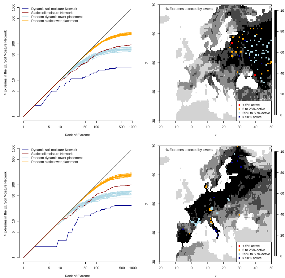
Figure D2. International Soil Moisture Network and its capacities to detect SPI extremes in Europe vs. a random network for the 1980ies (upper row) and 2000s (bottom row).
