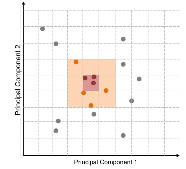
Figure A1. Illustration of identification of regions with similar threshold: We define a grid in the space of the leading PCs (geographically shown in Fig. 1), where each mesh width corresponds to 4% of the total min-max range of the first PC. We assign percentile thresholds as calculated over a 3 \times 3 \times 3 set of mesh elements (shown in orange) and assign these percentiles to the central dots (shown in red). For the sake of clarity, we illustrate the approach only in the space of the leading two PCs.
