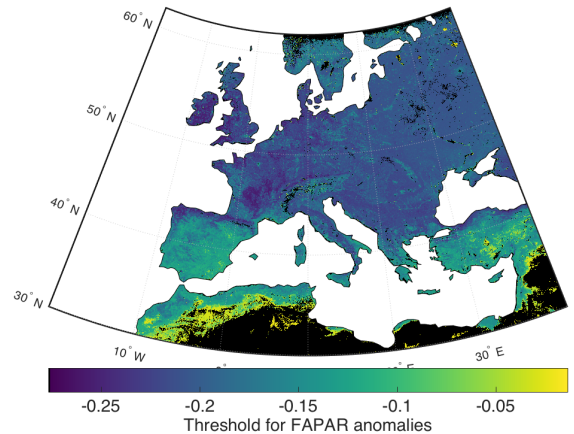
Figure 2. Map of the regionally varying FAPAR threshold used for detecting extreme events. These thresholds are derived within each subregion as defined by the leading PCs of the mean seasonal cycles. The gradient between central and southern Europe indicates that we may classify an event as extreme in one ecosystem that would be considered part of the normal variability elsewhere, i.e. arid ecosystems have lower thresholds of extremeness in FAPAR compared to humid areas.
