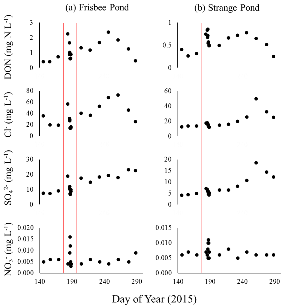
Figure 7. Short term variation in DON, Cl - , SO 4 2- , and NO 3 - concentrations in (a) Frisbee pond and (b) Strange pond during a rain event on July 3 rd to 6 th , 2015 (DOY 185-188, highlighted with red bars).
