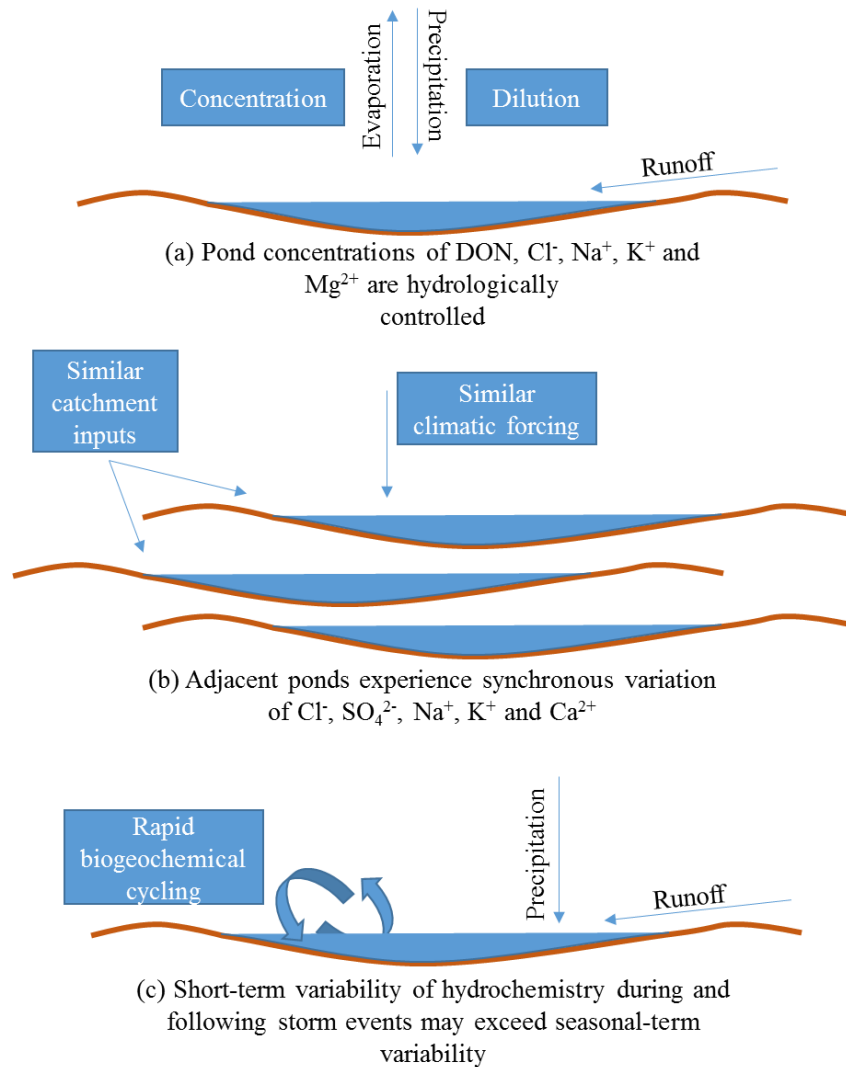
Figure 8. Graphical summation of major findings from this study; (a) factors driving hydrological control of particular chemical species in ponds, (b) hypothesised factors driving temporal coherence in chemical species in ponds, and (c) short-term variation in hydrochemistry can exceed seasonal-scale variation despite the large difference in timescales.
