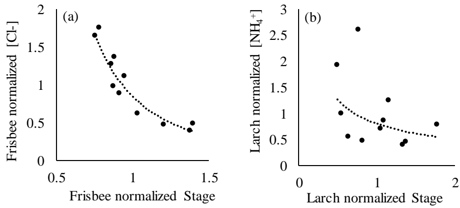
Figure 5: Comparison of the stage-concentration relationship in a) hydrologically driven chemical species ( Cl^- , in Frisbee pond), and b) a non-hydrologically driven species ( NH_4^+ , in Larch pond).
