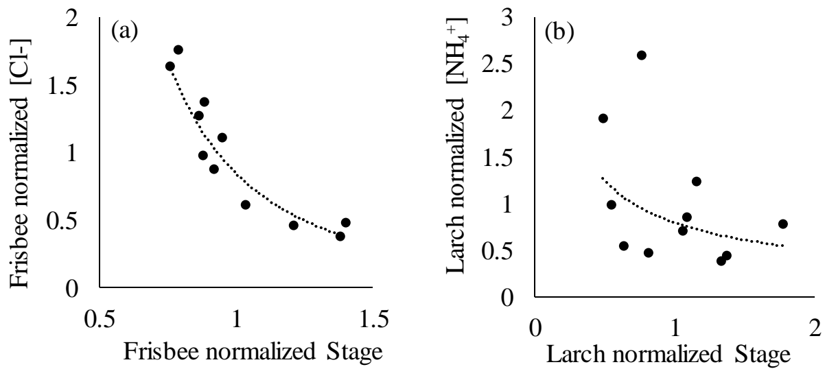
Figure 5: Comparison of the stage-concentration relationship in a (a) hydrologically driven chemical species ( \text{Cl}^- , in Frisbee pond), and (b) a non-hydrologically driven species ( \text{NH}_4^+ , in Larch pond).
