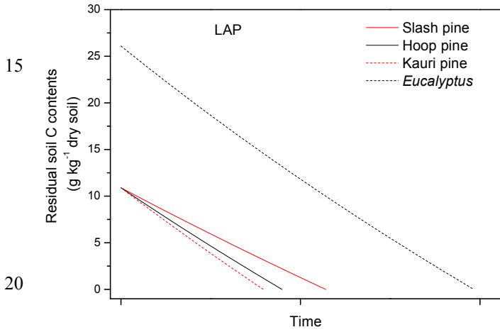
20 Figure 2. Residual soil C contents under different tree species across time for \beta -glucosidase (BG), N -acetylglucosaminidase (NAG), leucine aminopeptidase (LAP) and acid phosphatase (AP) at 25°C. The total soil C decomposition over time was calculated via Equation 5 and the residual soil C contents over time was compared for different enzyme activities among the tree species.
