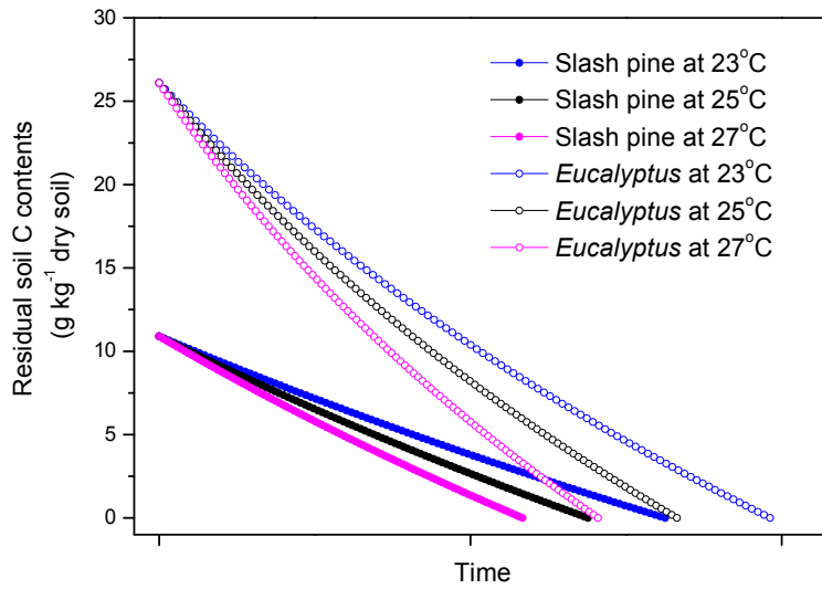
Figure 3. Residual soil C contents with \beta -glucosidase at 23°C, 25°C and 27°C under slash pine and Eucalyptus over time.
