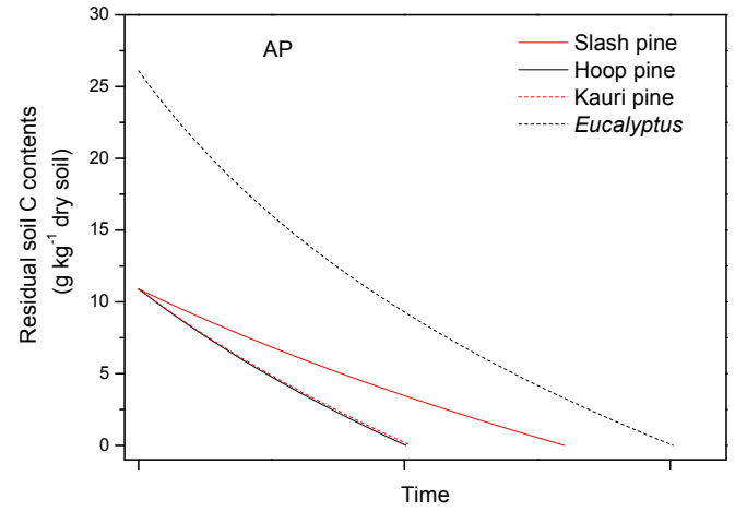
20 Figure 2. Residual soil C contents under different tree species across time for \beta -glucosidase (BG), N -acetylglucosaminidase (NAG), leucine aminopeptidase (LAP) and acid phosphatase (AP) at 25°C. The total soil C decomposition over time was calculated via Equation 5 and the residual soil C contents over time was compared for different enzyme activities among the tree species.
