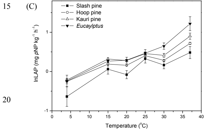
Figure 1. Extracellular enzyme activity in the soil along a gradient of temperatures under different tree species. (A) \beta -glucosidase (BG); (B) N -acetylglucosaminidase (NAG); (C) leucine aminopeptidase (LAP); (D) acid phosphatase (AP); p NP, para -nitrophenol.
