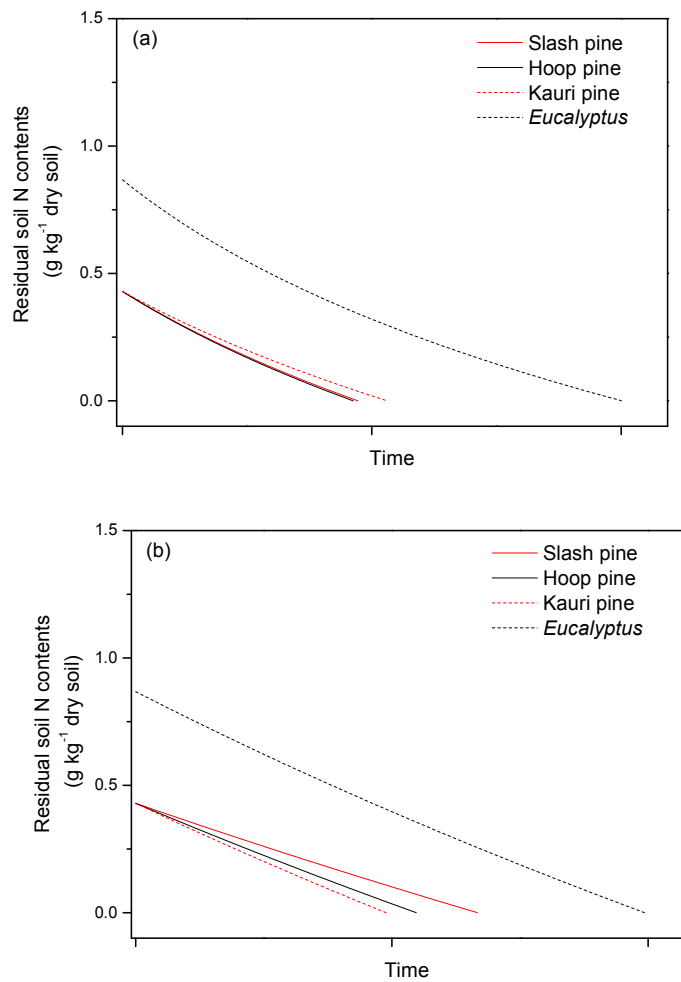
Figure 5. Residual soil N contents under different tree species with N -acetylglucosaminidase (a) and leucine aminopeptidase (b) across time. The total soil N decomposition over time was calculated via Equation 6 and the residual soil N contents over time was compared for different enzyme activities among the tree species.
