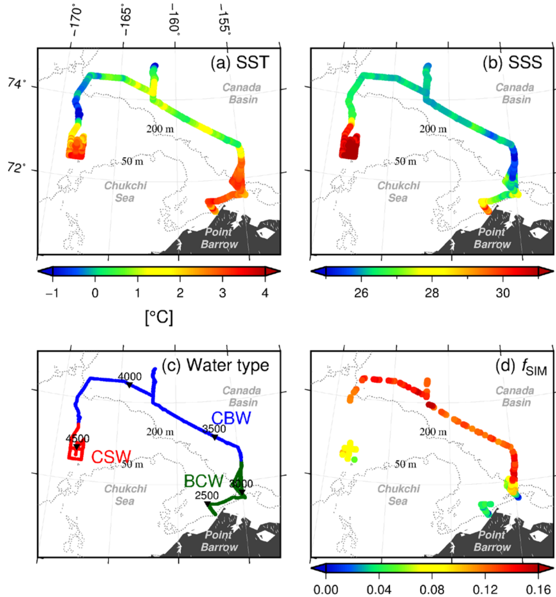
Figure 3: Surface water properties along the track of cruise MR13-06 from 4 to 11 September 2013. (a) Sea surface temperature (SST), (b) sea surface salinity (SSS), (c) BCW (Barrow Coastal Water), CSW (Chukchi Sea Water), and CBW (Canada Basin Water) water type according to SST and SSS. Number on triangles indicates distance sailed from Dutch harbor, Alaska, USA [km], (d) f_{SIM} , (e) f_{RRO} , (f) pCO_2^{sea} , (g) nDIC_{32} = DIC / S * 32 ; DIC normalized to S = 32 and (h) nTA_{32} = TA / S * 32 ; TA normalized to S = 32 . Dotted lines indicate 50 and 200 m isodepths.
