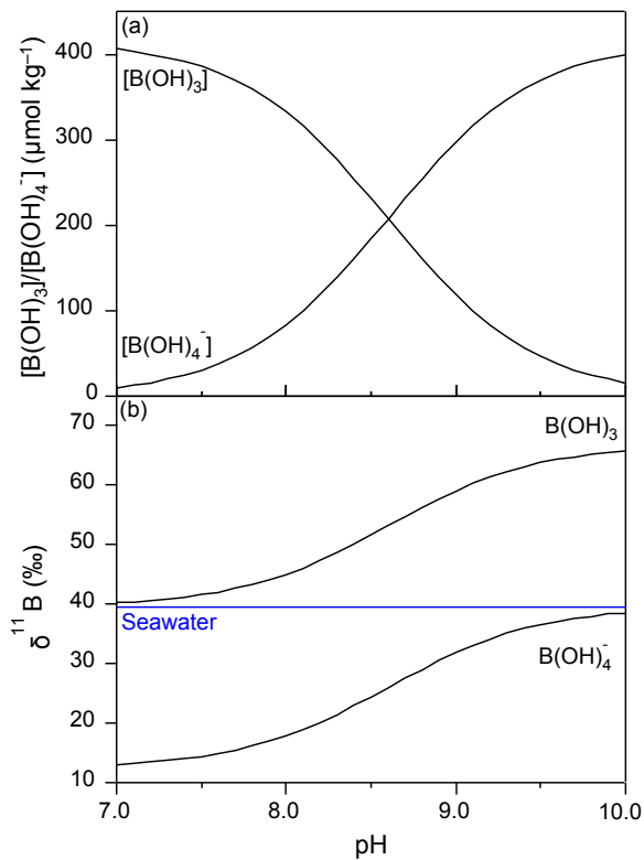
Figure 1. (a) Speciation of dissolved inorganic boron, \text{B}(\text{OH})_3 and \text{B}(\text{OH})_4^- , as a function of seawater pH. (b) \delta^{11}\text{B} of dissolved inorganic boron species as a function of seawater pH. The \text{pK}_\text{B} is 8.6 at 25 °C and 35 psu (practical salinity units; Dickson, 1990), \alpha is 1.0272 (Klochko et al., 2006), and \delta^{11}\text{B}_\text{SW} is 39.61 (Foster et al., 2010).
