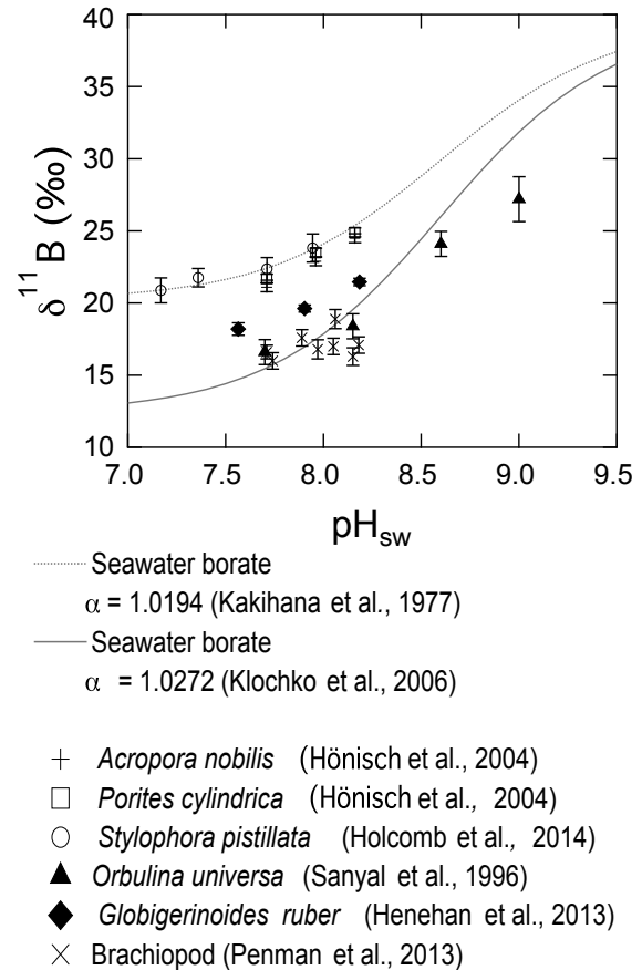
Figure 2. Examples of previously published \delta^{11}B_{CaCO_3} - pH_{sw} trends for corals, foraminifera, and brachiopods. Although many B isotope data sets are available, only studies with \geq 3 \delta^{11}B_{CaCO_3} - pH_{sw} data spanning a sufficiently wide range of pH_{sw} conditions were selected to illustrate the range of \delta^{11}B_{CaCO_3} - pH_{sw} trends published to date. The two grey lines correspond to the theoretical seawater borate \delta^{11}B -pH curves that have been applied most frequently to interpret \delta^{11}B variability in marine calcifiers. The pK_B is 8.6 at 25 °C and 35 psu (Dickson, 1990).
