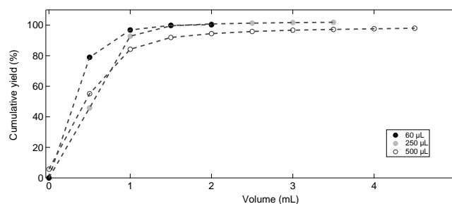
Figure 3. Elution curves indicating cumulative yield of boron for different volumes of the boron-specific resin (Amberlite IRA 743) used in the ion exchange column.
