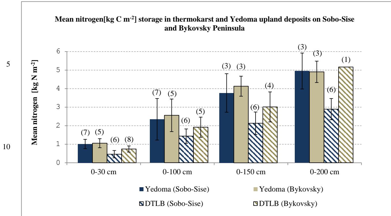
15 Figure 4: Mean sampling site N storage for the different geomorphic units in both study areas. Solid bars: Yedoma sites, striped bars: Thermokarst sites. Black T-lines show the standard deviation and number in brackets indicate the number of sampled sites. Profiles shorter than 200 cm were extrapolated to the next reference depth. When reaching an ice wedge in a collected site, this was included in the extrapolation as well, assuming no N for ice wedge layers. Soil N data for this graph are presented in the supplementary material, Table S1 and S5.
