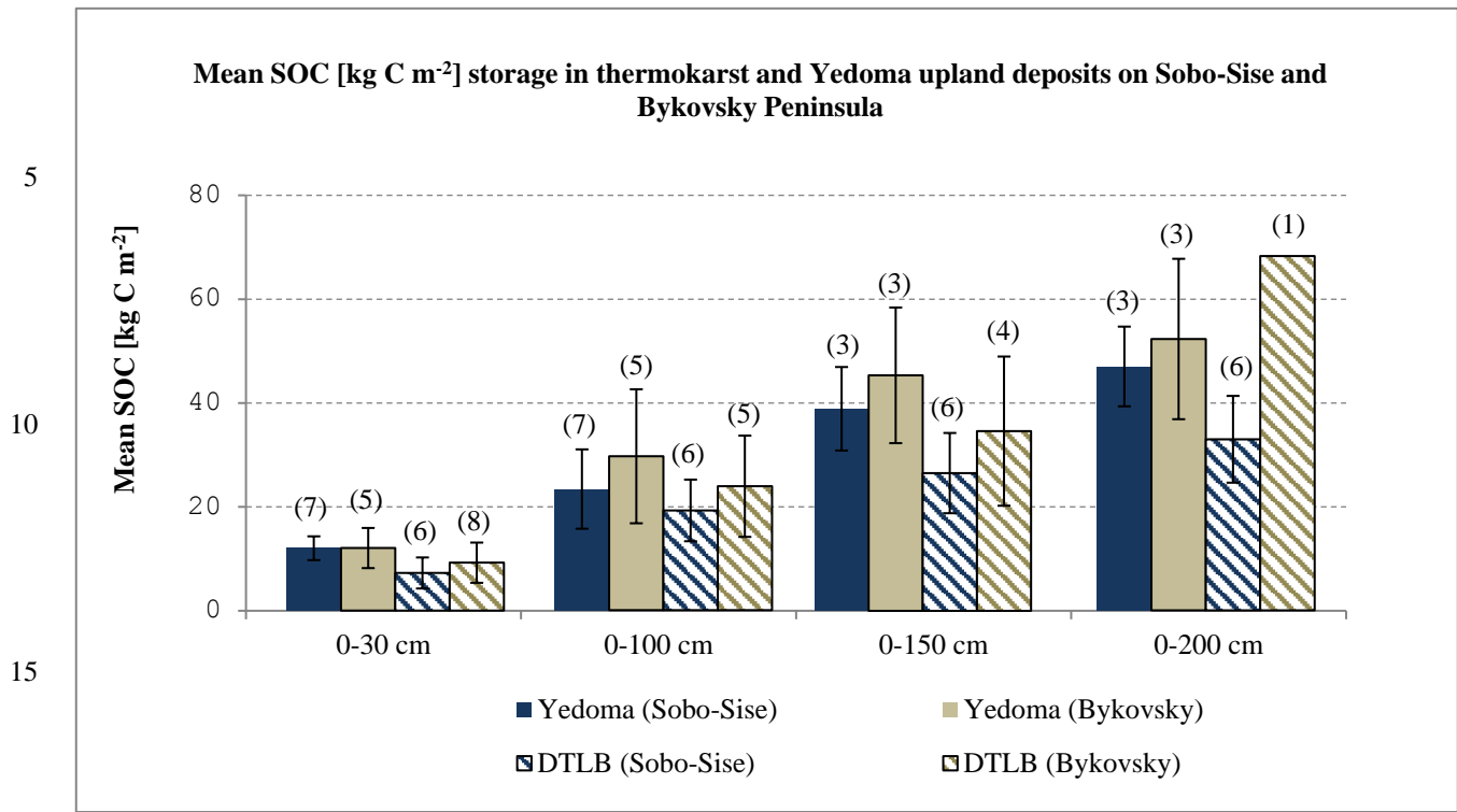
Figure 3: Comparison of mean sampling site SOC storage on Sobo-Sise Island and on Bykovsky Peninsula. Solid bars: Yedoma sites, striped bars: Thermokarst sites. Black T-lines show the standard deviation and number in brackets indicate the number of sampled sites. Profiles shorter than 200 cm were extrapolated to the next reference depth. When reaching an ice wedge in a collected site, this was included in the extrapolation as well, assuming no carbon for ice wedge layers. SOC data for this graph are presented in the supplementary material, Table S1 and S4.
