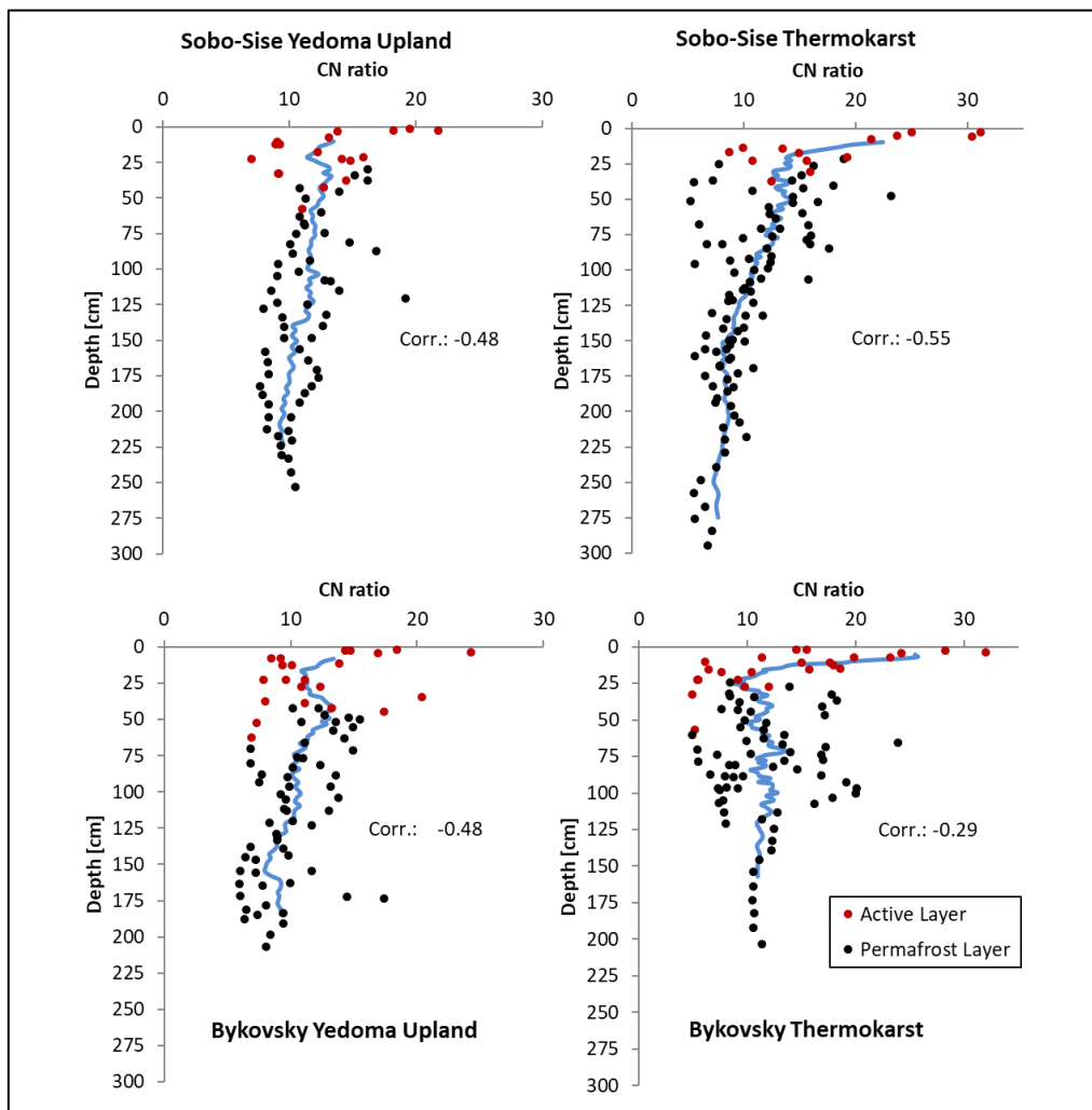
Figure 2: CN ratio for Yedoma upland and thermokarst samples on Sobo-Sise and Bykovsky Peninsula. Blue lines indicate the running mean for the entire sample set (including active layer and permafrost layer samples). The correlation (Corr.) (Pearson correlation) between CN ratio and depth indicates a decreasing CN ratio with increasing depth ( p < 0.01 ).
