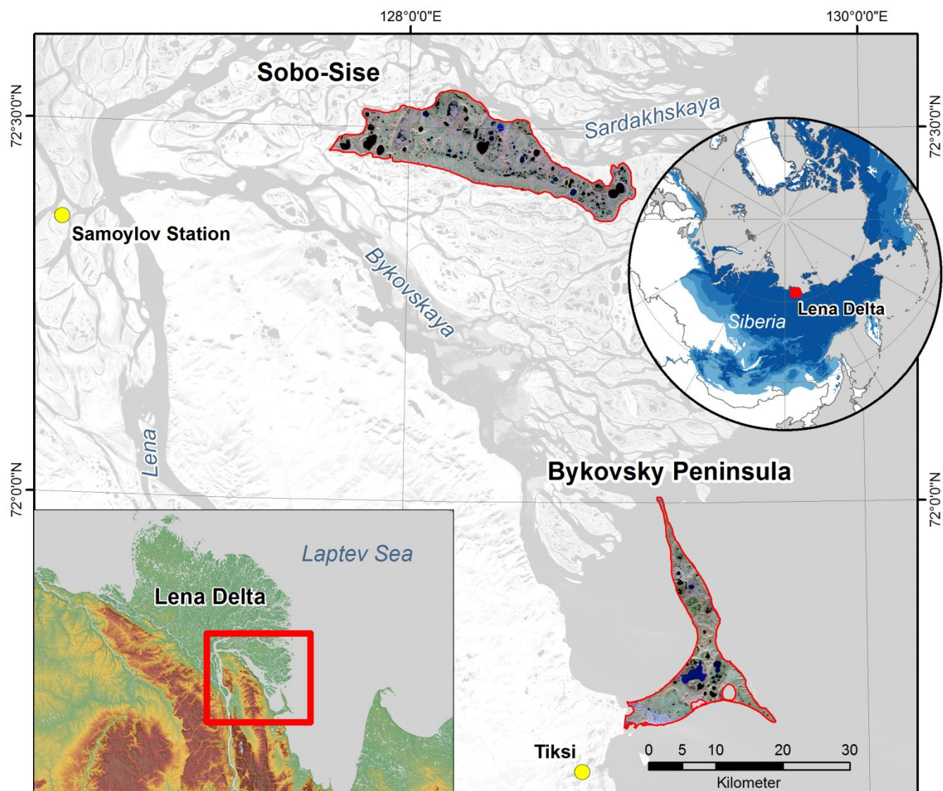
Figure 1: Location of the two study areas in the Lena River Delta region, Sobo-Sise Island and Bykovsky Peninsula (Landsat 5 satellite image, acquisition date: 19 th Sept. 2009). Top right inset: overview map including the permafrost zonation in Siberia (after Brown et al., 1997), bottom left inset: the Lena Delta region with a digital elevation model (ESA DUE-Permafrost DEM, Santoro and Strozzi, 2012).
