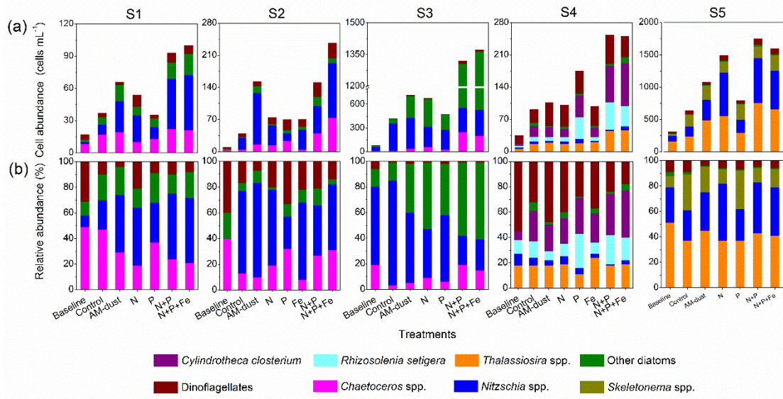
Figure 5. Changes in the taxonomic structure of large-sized phytoplankton community before (i.e., ‘baseline’) and during (i.e., ‘control’ and various treatments) the successive increase in the incubation period at each station. (a) Cell abundance of large-sized phytoplankton. (b) Relative abundance, i.e., the contribution of specific species to the large-sized phytoplankton community in cell abundance
