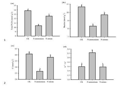
1 2 3 Fig.3 The effects of ammonium and nitrate additions on Total PLFAs, PLFA contents of bacteria, G 4 and G/G-. Small letters represent significant differences between treatments ( P < 0.05 ), error bars 5 represent means \pm standard errors ( n=9 ), G + represents gram positive bacteria and G - represents gram 6 negative bacteria.
