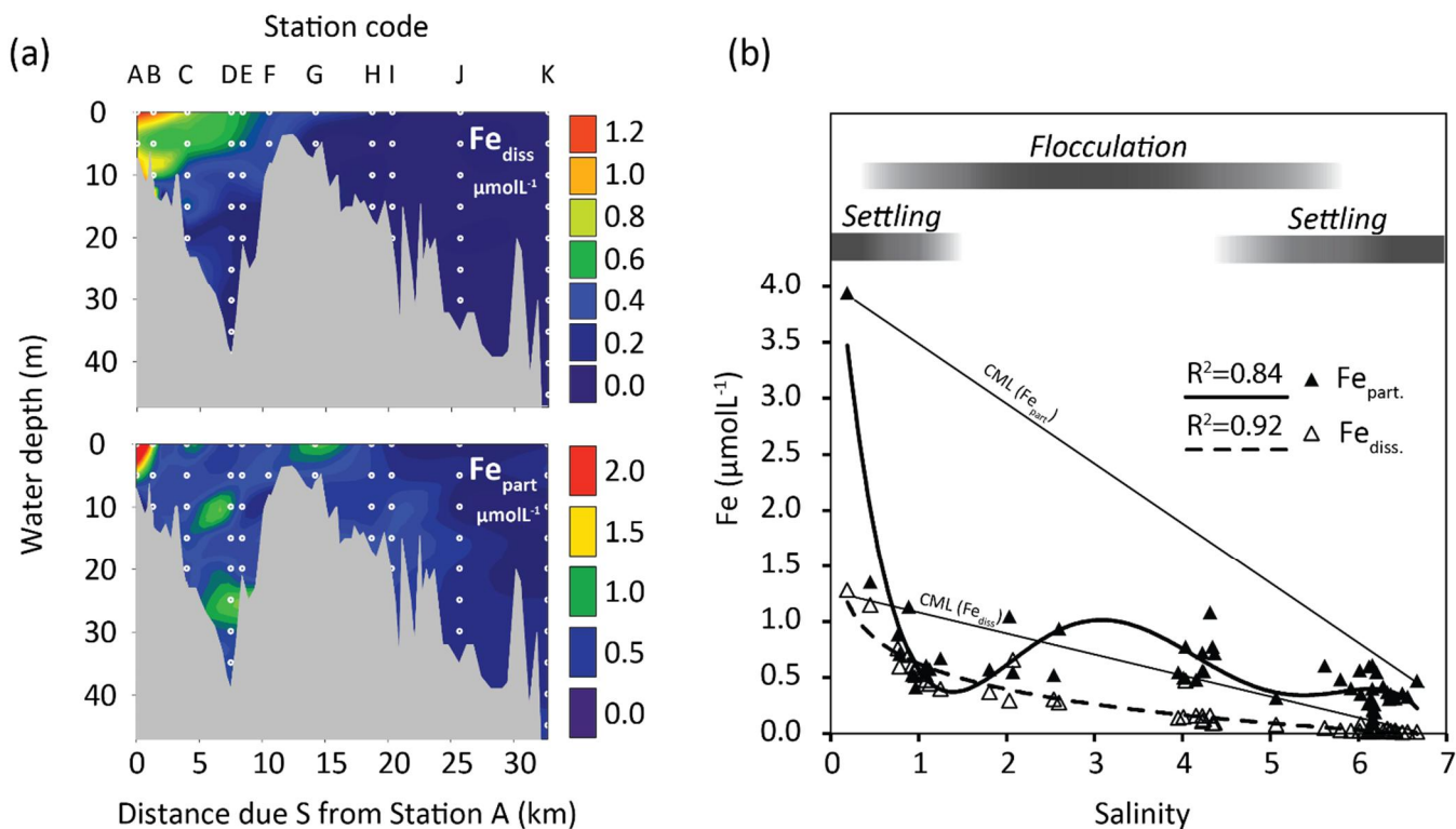
Figure 2. (a) 2D contour plots of dissolved (top) and particulate (bottom) Fe in the water column along the Mustionjoki transect (Stations A–K), operationally defined by filtration at 0.45 \mu m , June 2015. White circles represent sampling positions (vertical depth resolution = 5m). (b) Data from a plotted against salinity, including trendlines for Fe_{part} (polynomial) and Fe_{diss} (logarithmic). Linear Conservative Mixing Lines (CML) are drawn between the high- and low-salinity end-member samples for Fe_{part} and Fe_{diss} . The inferred dominant processes controlling Fe_{part} along the salinity transect are indicated by the grey bars.
