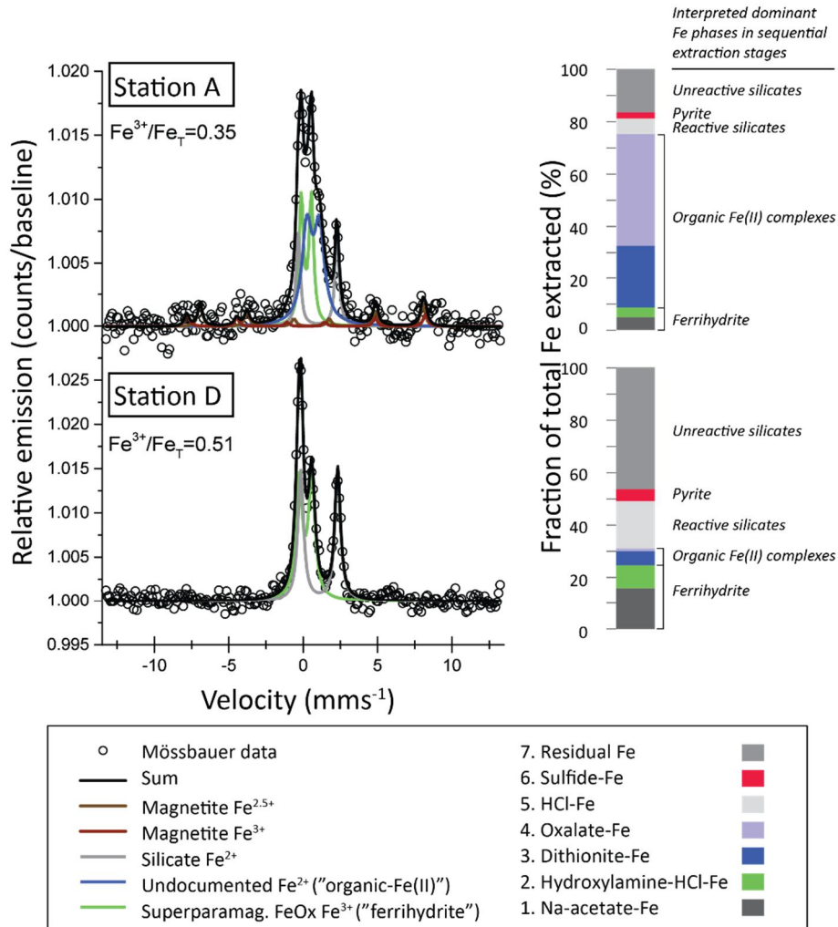
Figure 5. (left) Mössbauer spectra of powdered surface sediments (0–1 cm) from Stations A and D, sampled in 2015 (0.0 and 7.5 km respectively from the river mouth of the Mustionjoki transect). Sub-spectra of Fe-bearing sedimentary components (colored lines) were combined using a linear combination fitting (LCF) routine to generate a sum spectrum (black line) with the closest fit to the raw data (circles). Concentrations of each component, and Fe^{2+}/Fe_T ratios, were estimated from the LCF model. Mössbauer fitting parameters are listed in Table 3. (right) Sequential extraction results from the same samples, showing the complete speciation of Fe according to the method of Poulton and Canfield (2005) and an additional extraction for sulfide-bound Fe. The interpreted dominant Fe phases in each stage of the sequential extraction are given in the right column.
