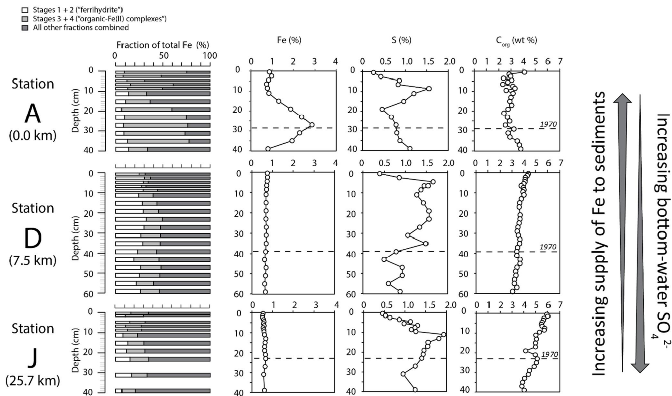
Figure 6. (left) Down-core operational Fe speciation for Stations A, D, and J (0.0, 7.5 and 25.7 km respectively from the river mouth of the Mustionjoki transect), derived from sequential extraction by the method of Poulton and Canfield (2005) and an additional extraction for sulfide-bound Fe. Thickness of bars corresponds to thickness of sampled interval (i.e. 1 or 2 cm). Note that not all depth intervals were sampled. (right) Down-core bulk chemical profiles from the same cores. Total Fe and S were determined by ICP-OES analysis of powdered sediments digested by HF+HClO_4+HNO_3 , while C_{org} was determined by thermal combustion of powdered sediments (see text for further details). The depth interval corresponding to 1970 is estimated from the peak in concentrations of total lead ( Pb_{tot} ) as determined by ICP-OES (see Supplementary information).
