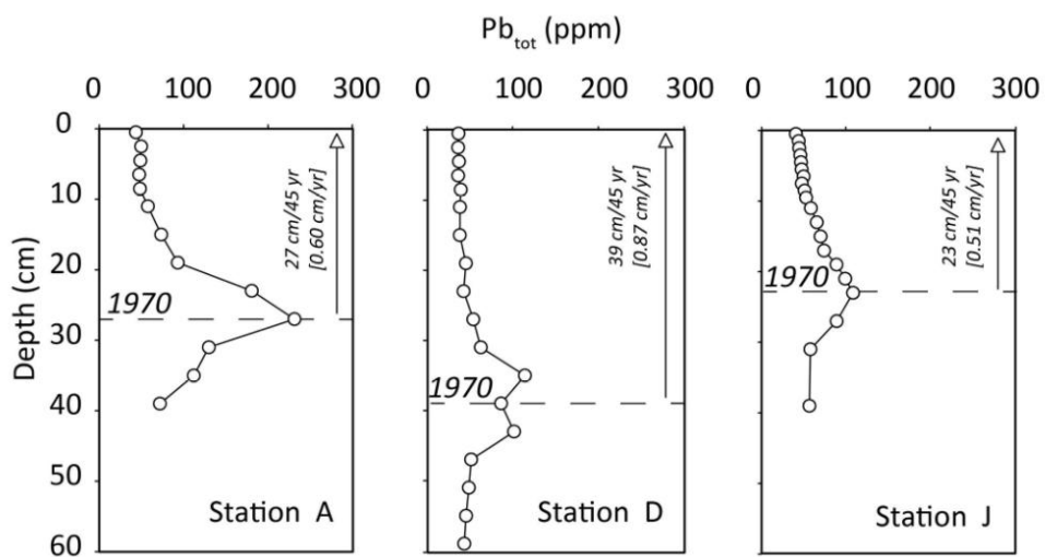
Supplementary Figure 1. Total lead ( Pb_{tot} ) concentrations in sediment cores from stations A, D and J in 2015, determined by ICP-OES. The peak in Pb_{tot} is assumed equivalent to the year 1970 (Zillen et al., 2012). Mean sedimentation rates for each core were estimated for the interval 1970-2015 as indicated in the panels.
