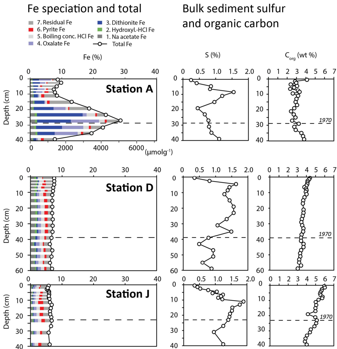
Figure 5. (left) Down-core operational Fe speciation and total sedimentary Fe content for Stations A, D, and J. Thickness of bars corresponds to thickness of sampled interval (i.e. 1 or 2 cm). Note that not all depth intervals were sampled. (right) Bulk chemical profiles from the same cores. The depth interval corresponding to 1970 is estimated from the peak in concentrations of total lead ( Pb_{tot} ) (see Supplementary Fig. 1).
