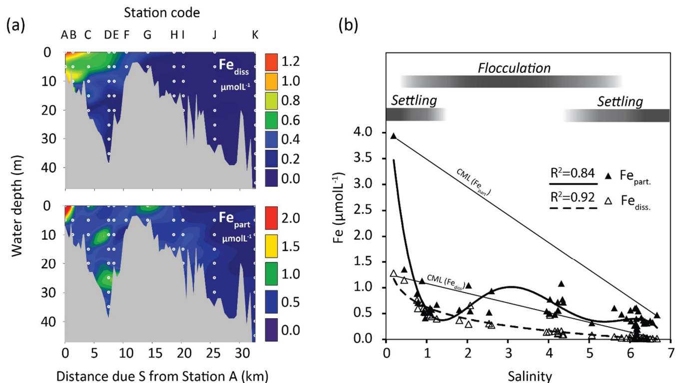
10 Figure 2. (a) 2D contour plots of dissolved (top) and particulate (bottom) Fe in the water column along the Mustionjoki transect (Stations A–K), operationally defined by filtration at 0.45 \mu\text{m} , June 2015. White circles represent sampling positions (vertical depth resolution = 5m). (b) Data from a plotted against salinity, including trendlines for \text{Fe}_{\text{part}} (polynomial) and \text{Fe}_{\text{diss}} (logarithmic). Linear Conservative Mixing Lines (CML) are drawn between the high- and low-salinity end-member samples for \text{Fe}_{\text{part}} and \text{Fe}_{\text{diss}} . The inferred dominant processes controlling \text{Fe}_{\text{part}} along the salinity transect are indicated by the grey bars.
