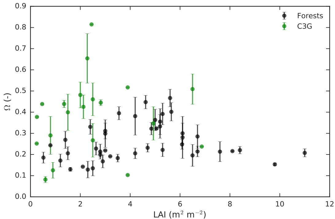
Fig. 1. Values of the estimated decoupling coefficient ( \Omega ) for forest (ENF, EBF, DBF, TRF) vegetation and C3 grasses as a function of LAI. Plant functional types are defined as: C3G - C3 grass, ENF - evergreen
