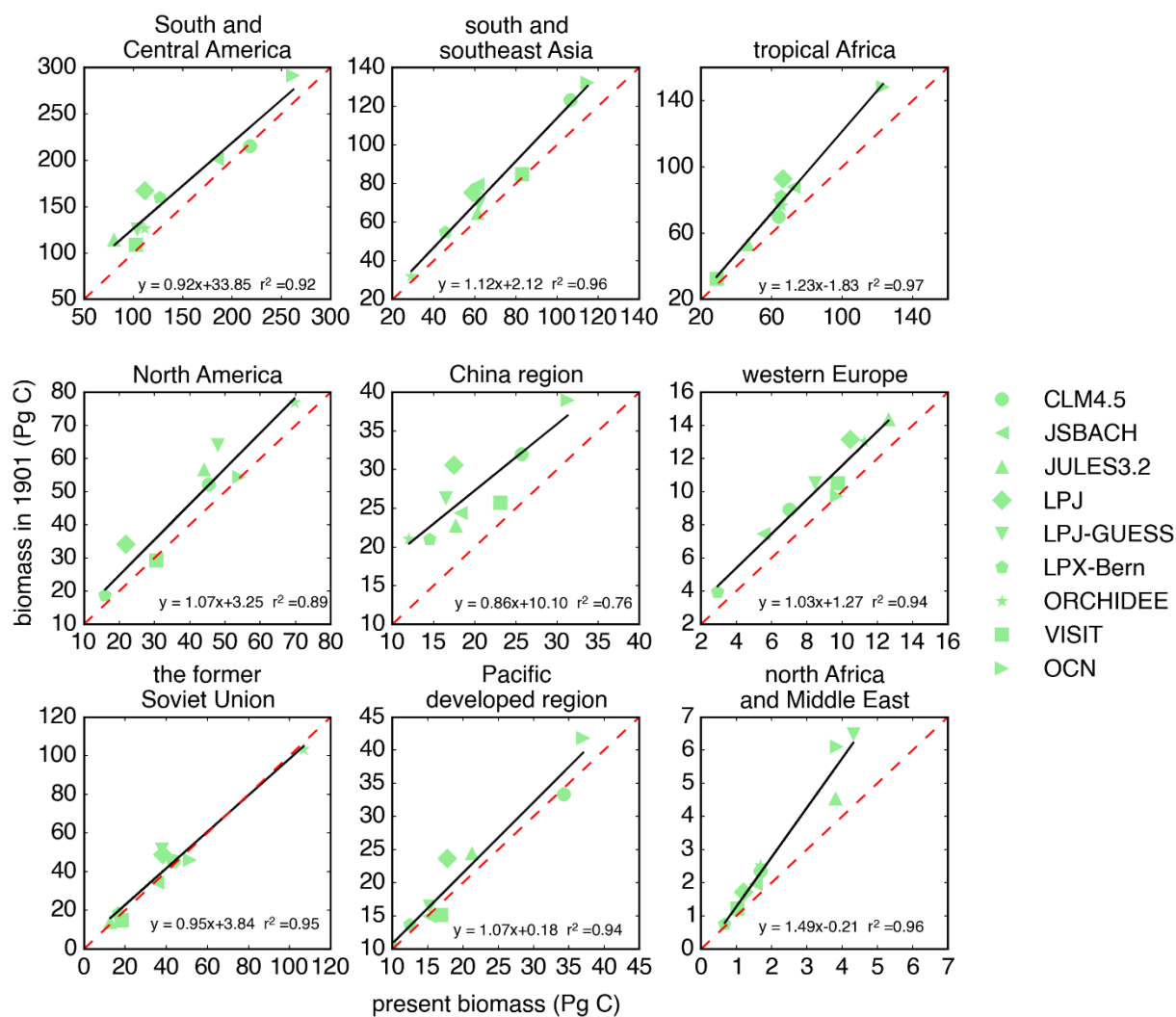
Figure 4. The relationship between initial biomass in 1901 and present biomass (average of biomass from 2000 to 2012) across the TRENDY v2 models for each region. Dashed line is the 1:1 line.
