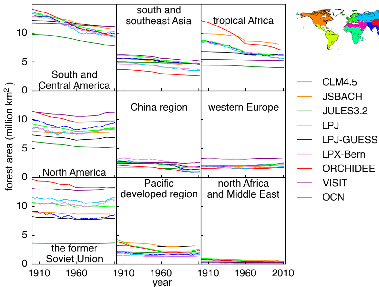
Figure 2. Temporal change of forest area from TRENDY v2 models in each of the nine regions. Differences between models arise from their specific vegetation maps and rules through which natural PFTs are chosen to give land to agriculture.
