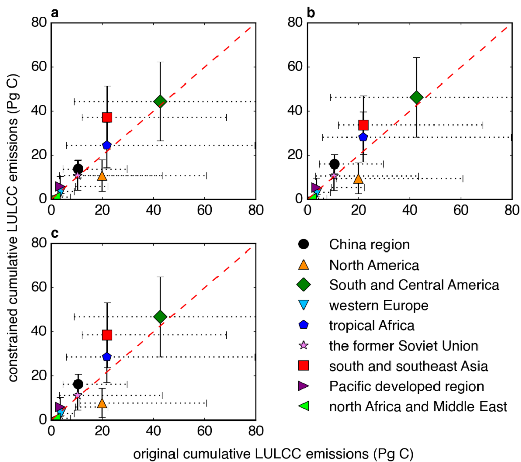
5 Figure 5. Comparisons between the original TRENDY land-use and land-cover change (LULCC) emissions and the cumulative LULCC emissions constrained by biomass dataset from Carvalhais et al. (2014). (a), (b) and (c) are results from Method-A, Method-B, and Method-C, respectively. Solid and dotted lines represent the 1- \sigma Gaussian error after biomass constraint and the original modeled range. Dashed line is the 1:1 line.
