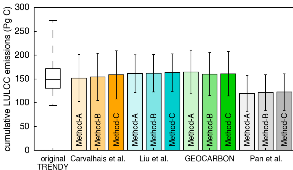
Figure 6. The global cumulative land-use and land-cover change (LULCC) emissions during 1901-2012 from original TRENDY models and from the estimates constrained by different biomass datasets with different methods to define deforestation grid cells. The whisker-box plot represents the minimum and maximum values, 25th and 75th percentiles and the median value of original TRENDY models. The error bars in the bar plot represent the 1- \sigma Gaussian errors.
