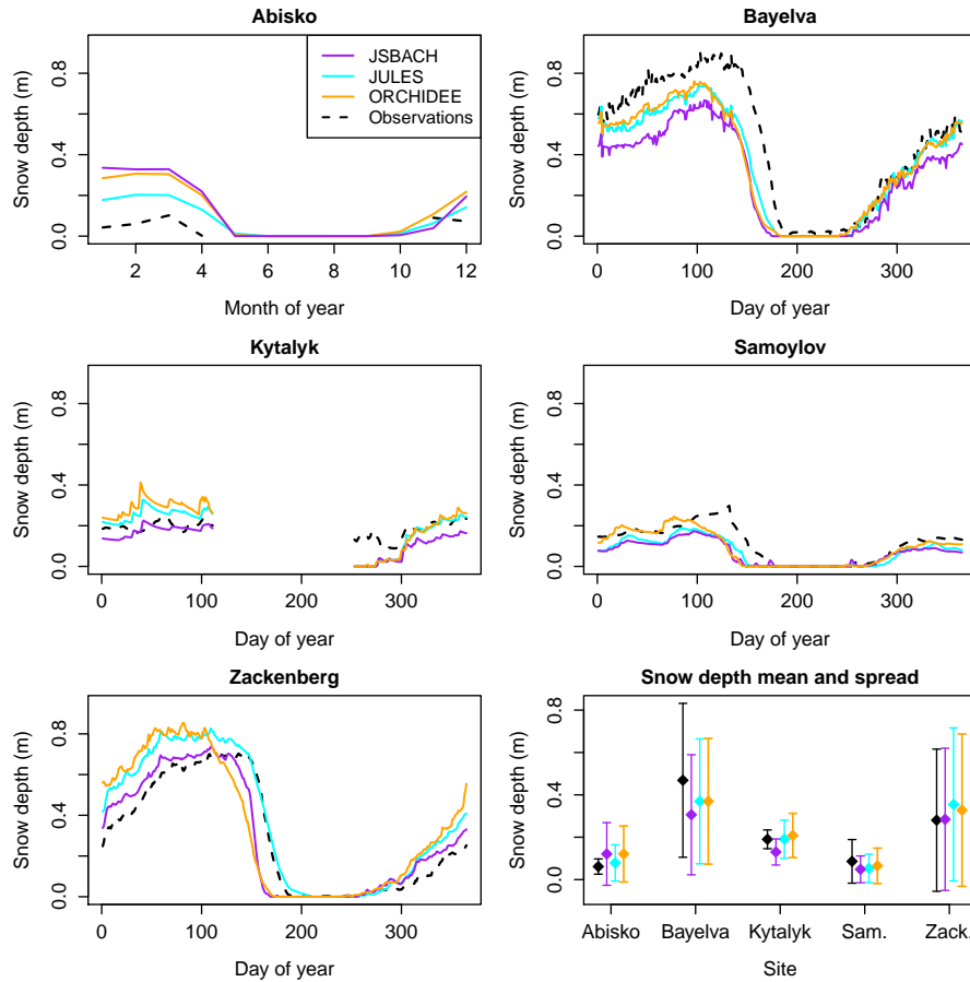
Figure 1. Mean annual cycle of snow depth at each site, showing both observations and models. On 6th panel, Samoylov and Zackenberg are abbreviated to ‘Sam.’ and ‘Zack.’ Mean annual cycle is calculated from a single site over a number of years, except for Abisko where measurements were taken in several different locations on the mire. See supplementary Table S1 for years used at each site.
