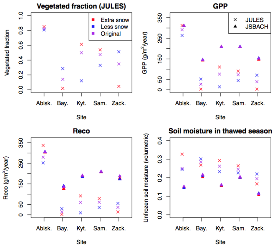
Figure S7 | Impacts of increased/reduced snowfall on soil moisture and carbon-cycle related variables (GPP, ecosystem respiration, and vegetated fraction), in JSBACH and JULES.
