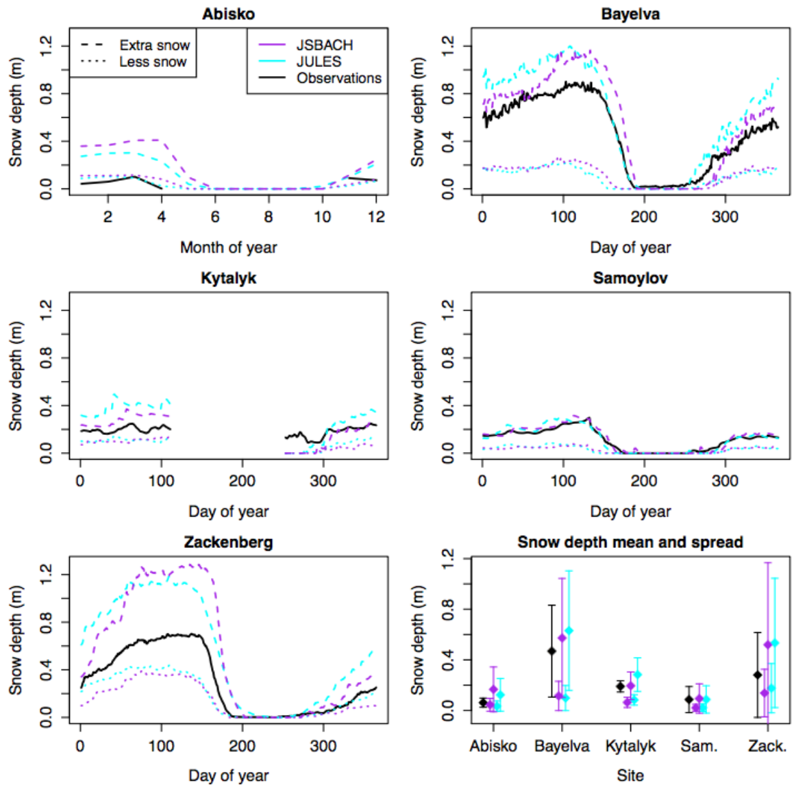
Figure S5 | Mean annual cycles of snow depth (as in Fig. 1 in main manuscript) showing simulations with increased and reduced snowfall in JSBACH and JULES.
