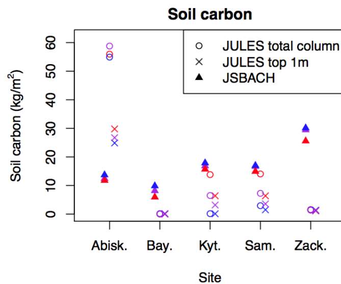
Figure S8 | Impact of increased/reduced snowfall on soil carbon stocks in JSBACH and JULES.
