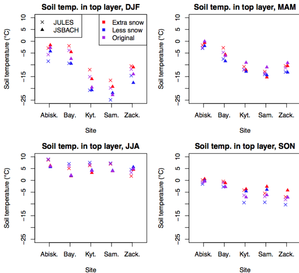
Figure S6 | Mean soil temperature in different seasons, showing simulations with increased and reduced snow for JULES and JSBACH. (DJF=December, January, February. MAM=March, April, May. JJA=June, July, August. SON = September, October, November.)
