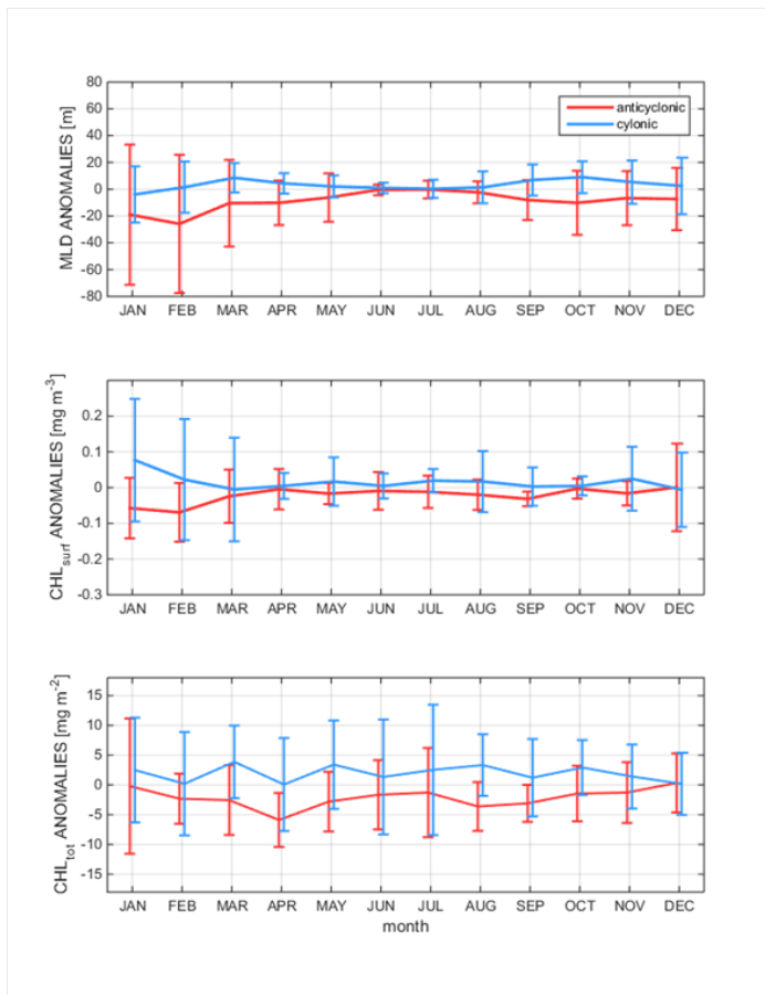
Fig. 2. Figure 2. Same as fig. 5 in the submitted manuscript but for anomalies: (top) the mixed layer depth, (middle) surface chlorophyll and (bottom) integrated chlorophyll over the first 350m.
