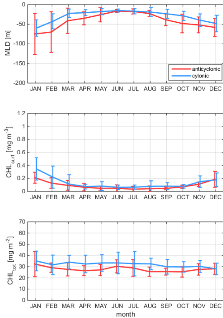
5 Figure 5: Basin-scale, monthly climatological mean and standard deviation of: (top) the mixed layer depth, (middle) surface chlorophyll and (bottom) integrated chlorophyll over the first 350m. Red (blue) shows statistics for all profiles in anticyclonic (cyclonic) structures.
