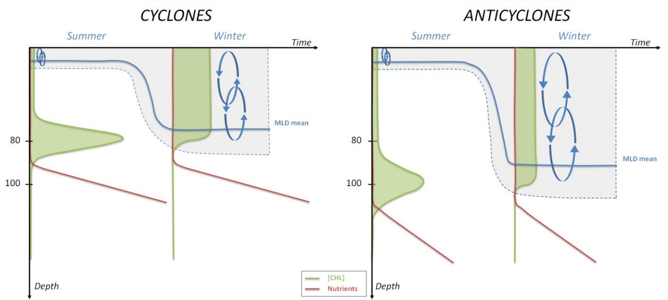
10 Figure 8: Conceptual view summarizing the basin-scale seasonal changes in the vertical distribution of chlorophyll (green), nutrients (red), mixed layer (shaded gray area) and mean mixed layer depth (blue), in cyclones and anticyclones. The total chlorophyll content is represented by the green area, which is approximately the same in summer than winter for either cyclones or anticyclones. By contrast, the chlorophyll content in cyclones is larger than in anticyclones for either season, showing that cyclones have slightly higher biomass. This may be the result of slightly higher nutrient supply in cyclones due to a steeper nutricline, and hence a higher diffusive flux. Finally, note that the mixed layer does not on average reach the nutricline in winter, but it does reach the deep chlorophyll maximum, resulting in the vertical redistribution of chlorophyll via vertical mixing and/or photoacclimation processes. 15
