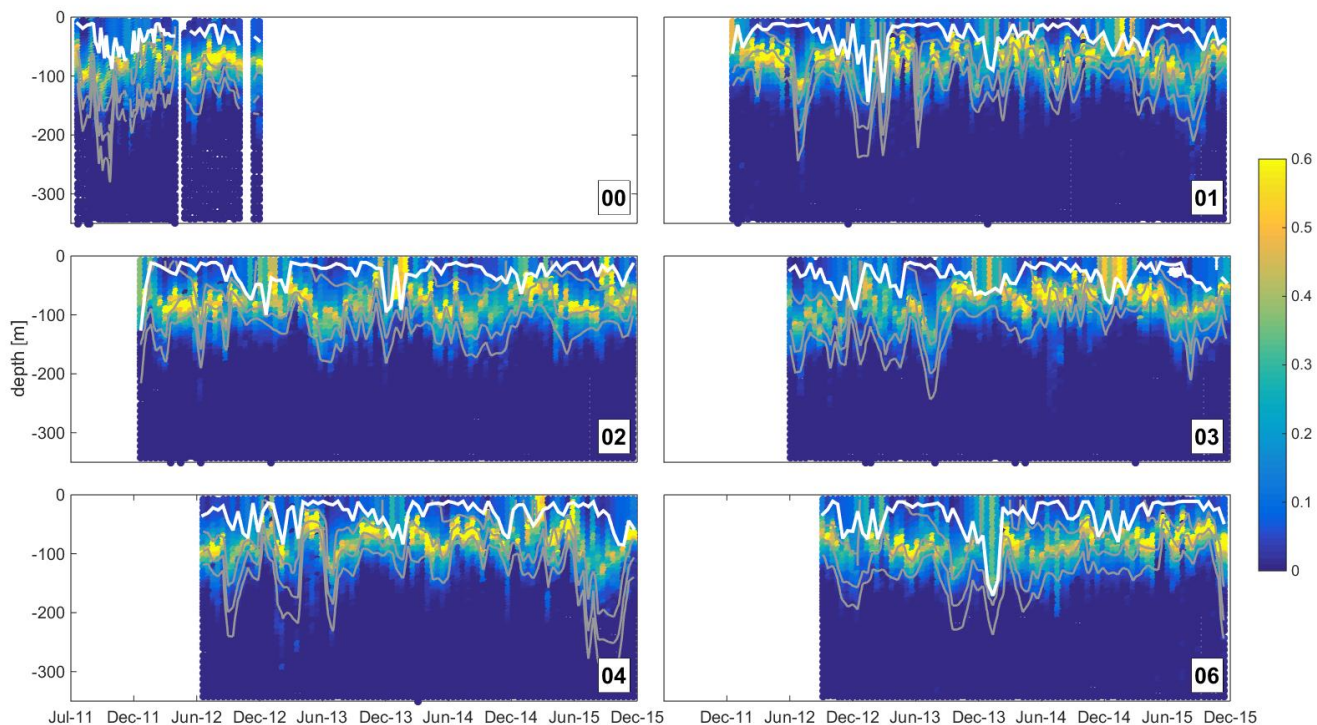
10 Figure 3: Calibrated [CHL] float transects in \text{mg m}^{-3} . Contour plots of density (1024.5 1025.5 1026 \text{kg m}^{-3} , grey lines), and mixed layer depth calculated as the depth where the difference of density from the surface reference, fixed at 10 m-depth, is 0.03 \text{kg m}^{-3} (solid white line), are superimposed.
