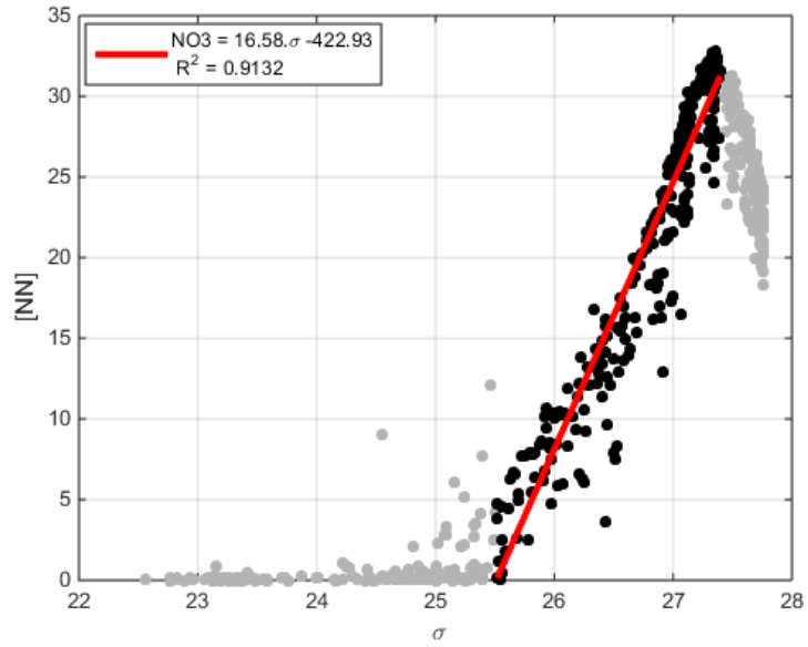
10 Figure 6: Nitrate + nitrite concentrations versus potential density anomaly data from XIXIMI-2 and XIXIMI-3 survey cruises. Measurements corresponding to the intermediate layer are plotted in black and were used for the determination of the linear fit (see text).
