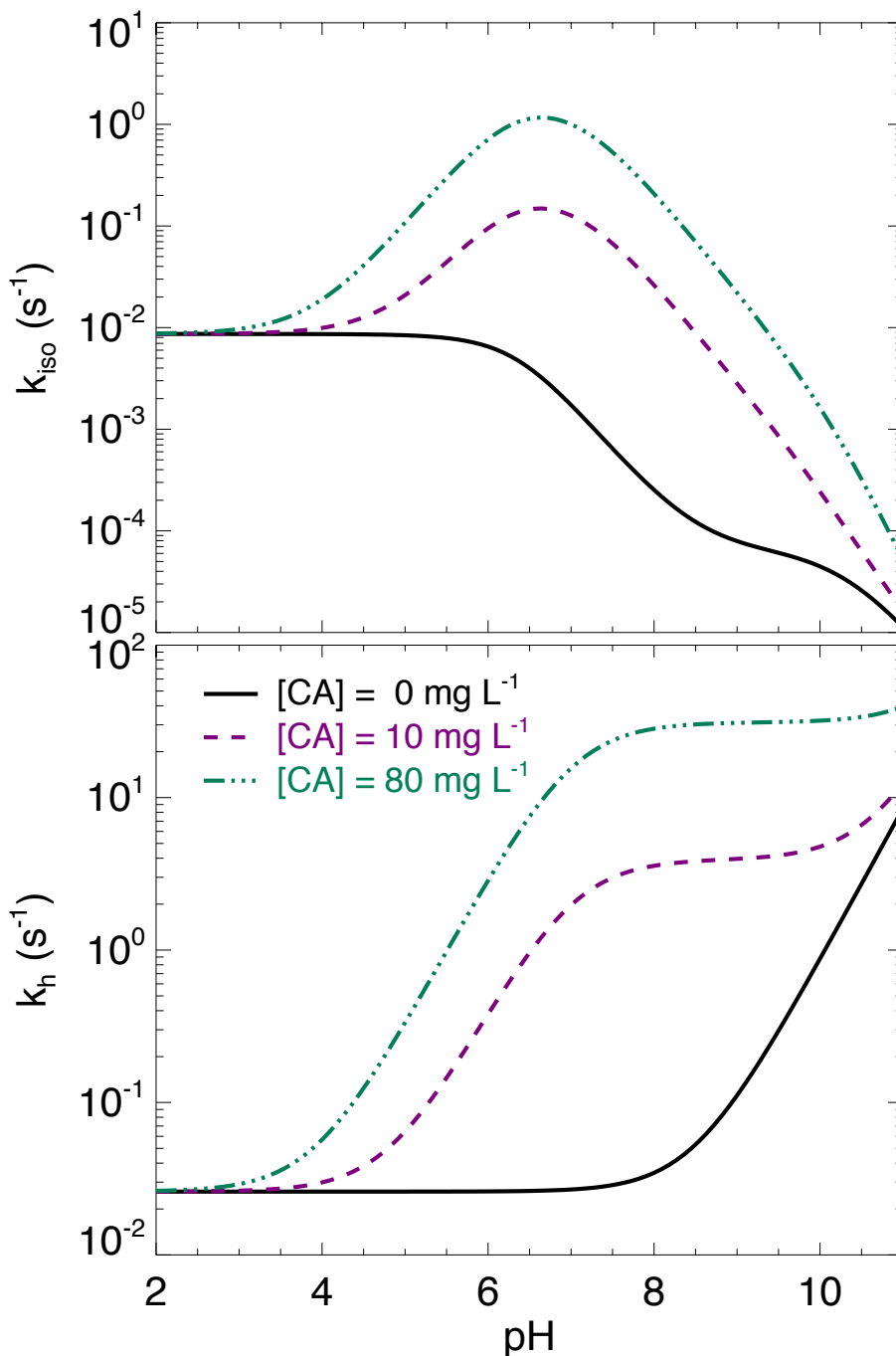
Figure 3: Theoretical rates of CO 2 hydration ( k_h ) and CO 2 -H 2 O oxygen isotope exchange ( k_{iso} ) as a function of pH, for 3 levels of carbonic anhydrase concentration. These theoretical curves have been obtained using the uncatalysed rate formula compiled in Uchikawa and Zeebe (2012) and enzymatic parameters of k_{cat}/K_M = 70 \text{ s}^{-1} \mu\text{M}^{-1} and pK_a = 7 , which are typical values for CA-catalysed CO 2 hydration (Rowlett et al., 2002; Smith and Ferry, 2000). Using enzymatic parameter values more specific to the \alpha -CA powder used here for the CA treatment (i.e. k_{cat}/K_M = 30 \pm 5 \text{ s}^{-1} \mu\text{M}^{-1} and pK_a = 7.1 \pm 0.5 ) would not change qualitatively this figure.
