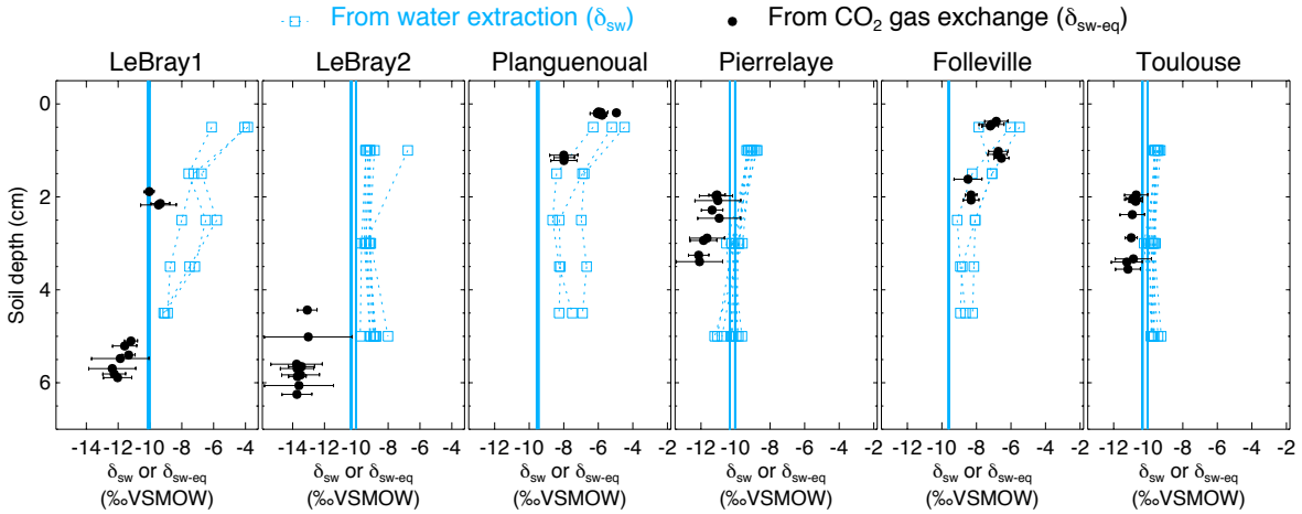
Figure 5: The isotopic composition of soil water at different depths in the replicated soil microcosms from each site, estimated either by vacuum distillation and water isotope analysis ( \delta_{sw} , blue squares) or online CO_2 - H_2O isotopic exchange using the two steady-state approach ( \delta_{sw-eq} , at depth z_{eq} , black circles, see text). Profiles for the different CA treatments are plotted together without distinction (because exogenous CA addition should not affect the isotopic composition of soil water). The blue vertical line also indicates the isotopic composition of the irrigation water used for the re-wetting of the air-dried soils. According to Eq.11, the addition of exogenous CA shifts the gas exchange results ( \delta_{sw-eq} ) to shallower depths ( z_{eq} ).
