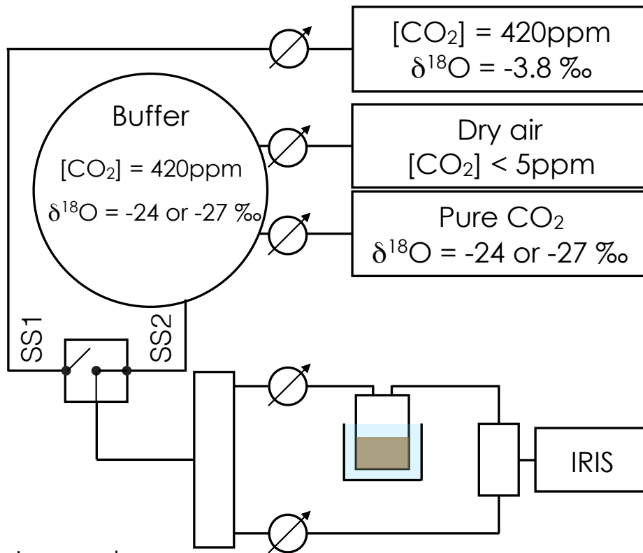
Figure 1: Schematic of the experimental setup used to estimate simultaneously the CO 2 -H 2 O isotope exchange rate ( k_{iso} ) in a soil microcosm and the oxygen isotopic composition of the soil water pool with which the CO 2 equilibrates ( \delta_{sw-eq} ). The soil microcosm consists of 280-300g of dry soil previously re-humidified to 25% of the water holding capacity using mineral water containing different amounts of exogenous CA powder. The soil column is thermally regulated using a 6.5L water bath and the air entering the chamber is a mixture of CO 2 in dry air whose oxygen isotopic composition is alternatively enriched (steady state 1, -3.8‰ VPDB g ) and depleted (steady state 2, between -24‰ and -27‰ VPDB g , depending on the experiment).
