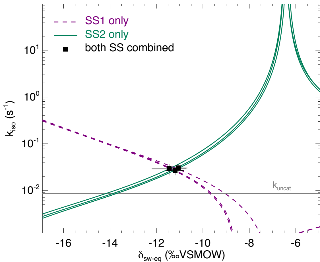
Figure 4: The CO 2 -H 2 O isotopic exchange rate ( k_{\text{iso}} ) and isotopic composition of soil water equilibrated with CO 2 ( \delta_{\text{sw}} ) retrieved using the two-steady-state approach described in the main text (Eqs. 6a and 6b), for one single microcosm (LeBray1 with an \alpha -CA addition of 24 mg L -1 ). Relationships between k_{\text{iso}} and \delta_{\text{sw}} for steady-state 1 (dotted lines) and steady-state 2 (solid lines) are also shown. In this example the microcosm was measured over 3 consecutive sequences, resulting in 3 curves for each steady state and 3 intersection points that coincide well with the two steady-state solution for each sequence (black squares). The pH-dependent, uncatalysed CO 2 -H 2 O isotopic exchange rate (Uchikawa and Zeebe, 2012) is also indicated by the grey horizontal line.
