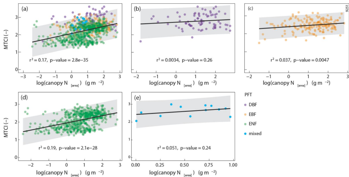
Figure 6. Scatterplot and log-linear regression line between the MERIS Terrestrial Chlorophyll Index (MTCI) (-) and canopy N content (canopy N [area] , g m -2 ) for (a) whole dataset (n = 841); (b) Deciduous Broadleaf Forest plots (DBF, n = 80); (c) Evergreen Broadleaf Forest plots (EBF, n = 186); (d) Evergreen Needleleaf Forest plots (ENF, n = 563); (e) mixed forest plots (n = 12). PFT = Plant functional type. The grey shading represents the prediction intervals (95 %). Canopy N [area] variable was log transformed to fulfil linear models assumptions.
