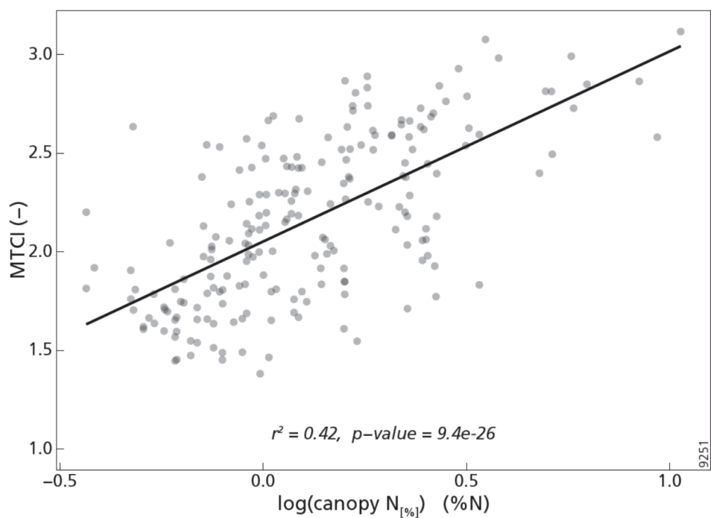
720 Figure 4. Scatterplot between the MERIS Terrestrial Chlorophyll Index (MTCI) (-) and canopy nitrogen concentration (canopy N_{[\%]} , %N) after resampling the datasets to 20 km-spatial resolution (n = 204).
