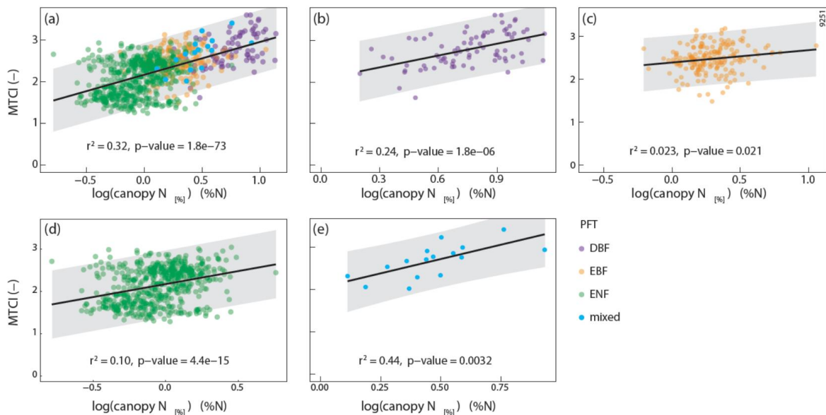
Figure 5. Scatterplot and log-linear regression line between the MERIS Terrestrial Chlorophyll Index (MTCI) (–) and canopy nitrogen (N) concentration (canopy N [%] , %N) for (a) whole dataset (n = 846); (b) Deciduous Broadleaf Forest plots (DBF, n = 80); (c) Evergreen Broadleaf Forest plots (EBF, n = 186); (d) Evergreen Needleleaf Forest plots (ENF, n = 564); (e) mixed forest plots (n = 16). PFT = Plant functional type. The grey shading represents the prediction intervals (95 %). Canopy N [%] variable was log transformed to fulfil linear model assumptions.
