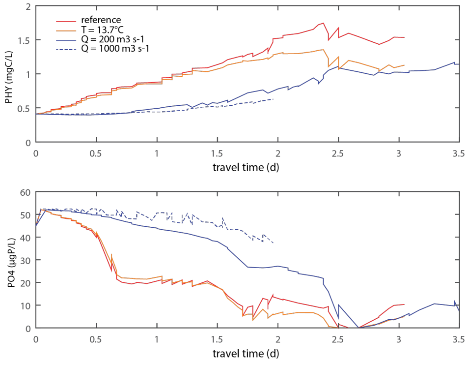
Fig. 3. Figure A3. Lagrangian view from S1 to S2 of phytoplankton and PO4 concentrations for 4 different scenarios
