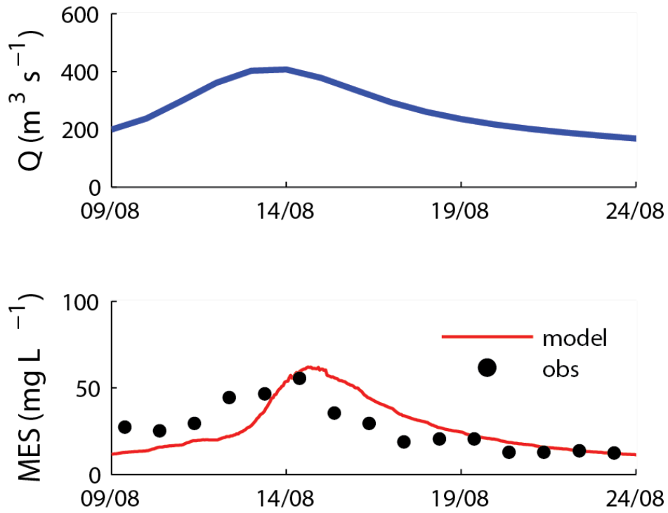
Fig. 6. Figure A6. Discharge and observed and modeled TSS concentration during the selected storm event
