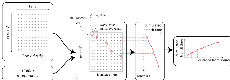
Fig. 5. Figure A5. Successive steps to produce Lagrangian longitudinal profiles
