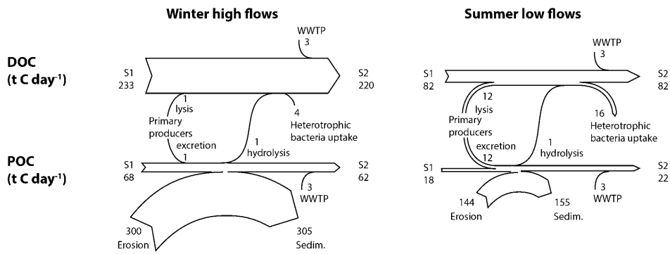
Fig. 4. Figure A4. DOC and POC budgets assessed with QUAL-NET between S1 and S2 (would be included in Figure 7)
