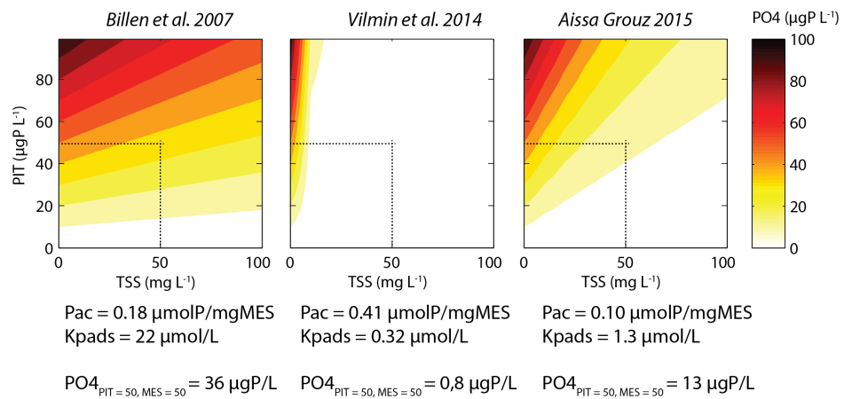
Fig. 7. Figure A7. Sensitivity of PO_4 estimations from total inorganic P (PIT) and suspended solids concentrations (MES) based on the Langmuir equilibrium concept
