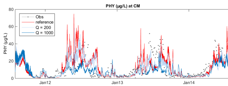
Fig. 1. Figure A1. Phytoplankton simulation sensitivity to hydrological conditions
