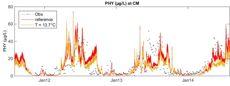
Fig. 2. Figure A2. Phytoplankton simulation sensitivity to water temperature conditions
