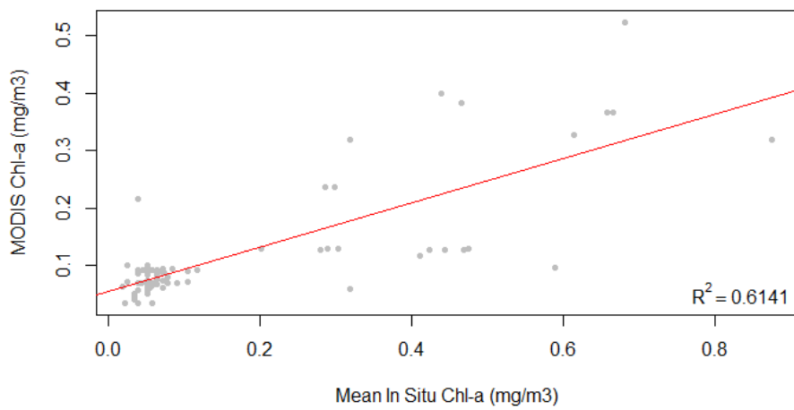
Fig. 2. The relationship between the in situ chlorophyll a concentrations measured from NOAA WOD and the MODIS chlorophyll a concentration product during times of TC absence in the area.
