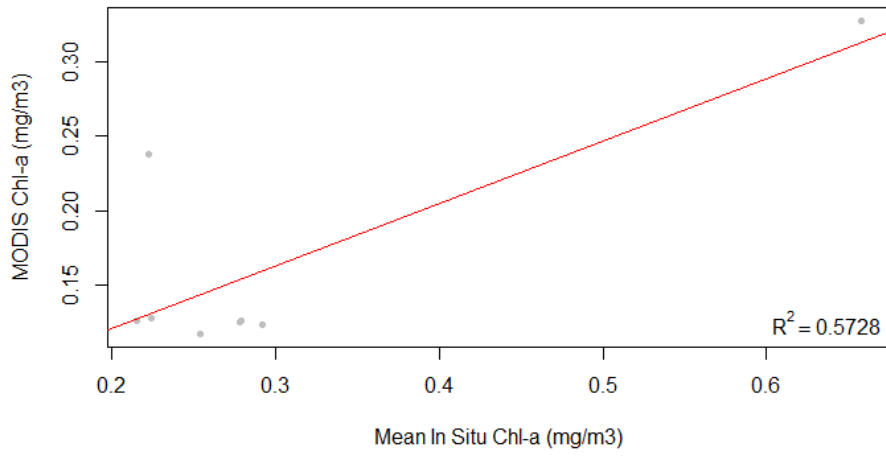
Fig. 1. The relationship between the in situ chlorophyll a concentrations measured from NOAA WOD and the MODIS chlorophyll a concentration product during times of TC presence in the area.
