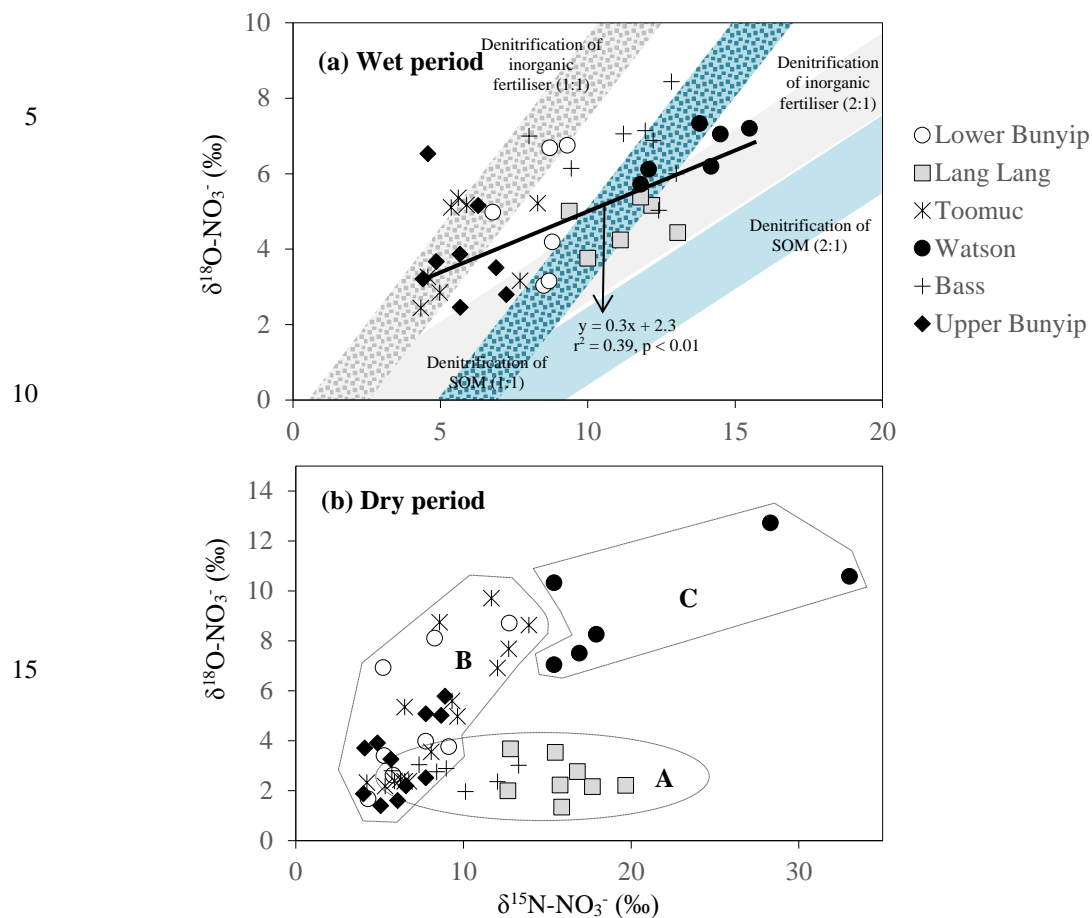
Figure 8: Biplot of \delta^{15}\text{N-NO}_3^- versus \delta^{18}\text{O-NO}_3^- for (a) wet and (b) dry periods. Blue shaded area represents possible isotopic compositions of denitrified \text{NO}_3^- originated from SOM ( \delta^{15}\text{N}: +4.5\text{‰} ). Grey shaded area represents the possible isotopic composition of denitrified \text{NO}_3^- originated from inorganic fertiliser ( \delta^{15}\text{N-NO}_3^-: +0.1\text{‰} ). The \delta^{18}\text{O-NO}_3^- used were -2.3\text{‰} and +0.23\text{‰} representing the minimum and maximum estimates of \delta^{18}\text{O} of nitrified \text{NO}_3^- , respectively. The shaded area were plotted based on the theoretical 1:1 and 2:1 denitrification relationships between \delta^{15}\text{N-NO}_3^- and \delta^{18}\text{O-NO}_3^- (Kendall et al. 2007).
