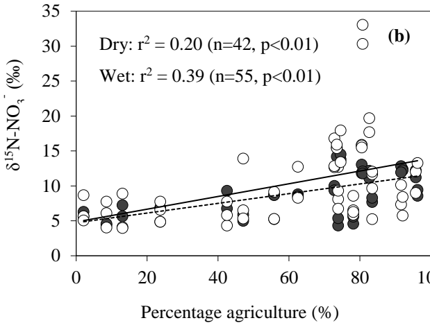
Figure 4: Relationship between (a) \text{NO}_3^- concentration; (b) \delta^{15}\text{N-NO}_3^- and the percentage of agricultural land use. In (b) solid line represents the relationship between the variables during dry periods; dotted line represents wet periods.
