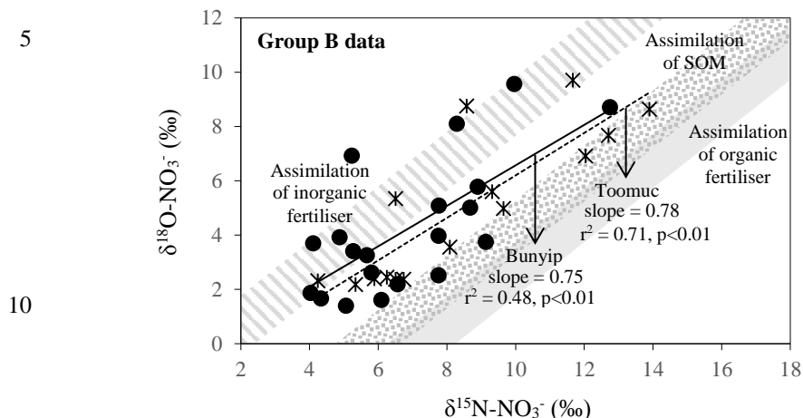
Figure 9: Biplot of \delta^{15}\text{N-NO}_3^- versus \delta^{18}\text{O-NO}_3^- for Bunyip and Toomuc (group B data in Fig. 8b). Shaded areas represent theoretical assimilation trends for cow manure, SOM and inorganic fertiliser. The maximum and minimum starting values for \delta^{18}\text{O-NO}_3^- were estimated from Equation 1. The starting \delta^{15}\text{N-NO}_3^- is the \delta^{15}\text{N-TN} value of respective end member. Solid and dotted lines represent the assimilation trends for Bunyip (both lower and upper Bunyip) and Toomuc, respectively. Assimilation rather than denitrification was considered a more plausible process controlling the distribution pattern for the group B dataset as the water column was oxic throughout the study period.
