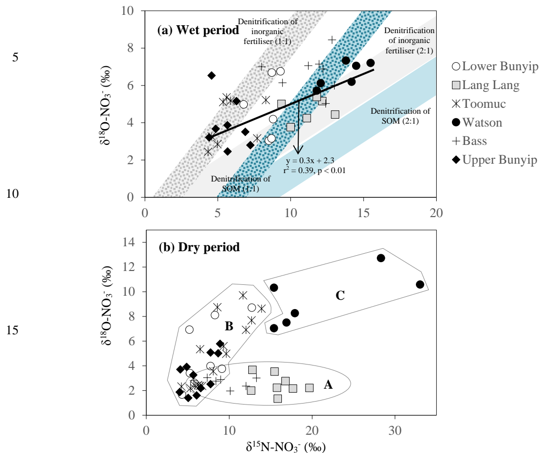
Figure 8: Biplot of \delta^{15}\text{N-NO}_3^- versus \delta^{18}\text{O-NO}_3^- for (a) wet and (b) dry periods. Blue shaded area represents possible isotopic compositions of denitrified \text{NO}_3^- originated from SOM ( \delta^{15}\text{N}: +4.5\text{‰} ). Grey shaded area represents the possible isotopic composition of denitrified \text{NO}_3^- originated from inorganic fertiliser ( \delta^{15}\text{N-NO}_3^-: +0.1\text{‰} ). The \delta^{18}\text{O-NO}_3^- used were -2.3\text{‰} and +0.23\text{‰} representing the minimum and maximum estimates of \delta^{18}\text{O} of nitrified \text{NO}_3^- , respectively. The shaded area were plotted based on the theoretical 1:1 and 2:1 denitrification relationships between \delta^{15}\text{N-NO}_3^- and \delta^{18}\text{O-NO}_3^- (Kendall et al. 2007).
