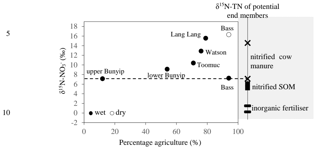
15 Figure 7: Relationship between \delta^{15}\text{N-NO}_3^- of the dominant initial source (indicated by the y-intercept of the Keeling plots; Figure 6) and percentage agriculture during wet periods. Data for Bass-dry period was also presented because only the Keeling plot for Bass-dry period indicates mixing between different sources. The shaded area represents the \delta^{15}\text{N-TN} of the potential end members.
