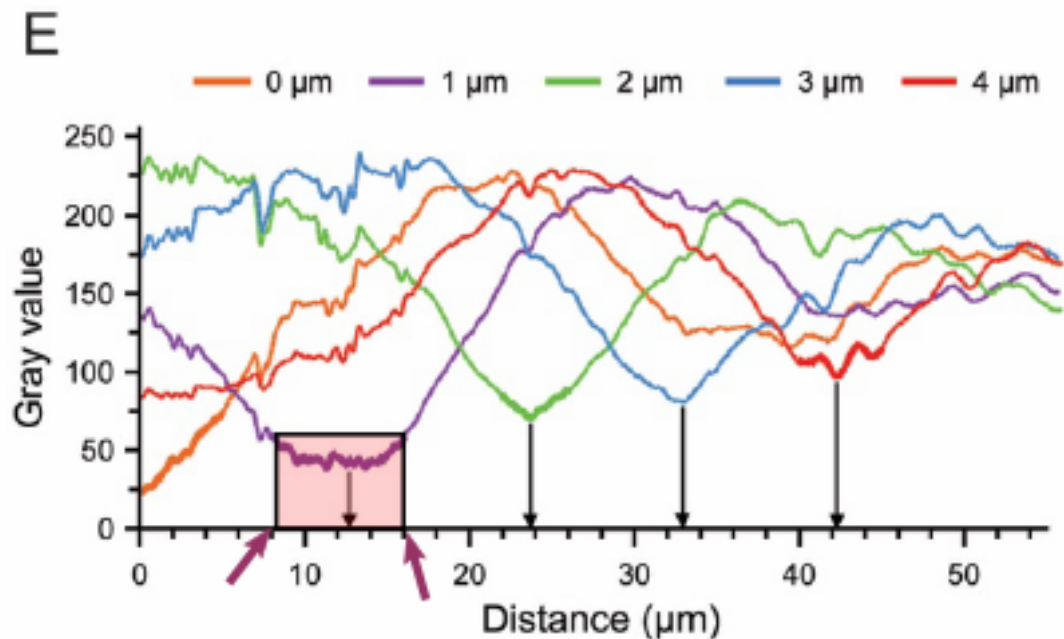
Fig. 1. Figure 2E from González-Lemos et al. (2017) with minimum area for 1 \mu\text{m} thickness of calcite wedge highlighted by the pink box. The black arrow in the pink box shows the distance position of \sim 12.5 \mu\text{m} on
