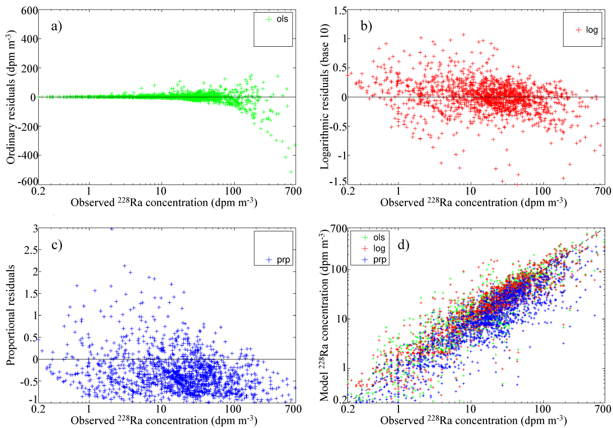
Figure 6. (a) Residuals, (b) logarithmic residuals, (c) proportional residuals and (d) model ^{228}\text{Ra} concentration as a function of observed ^{228}\text{Ra} concentration. Lines of zero residuals are drawn in black.
