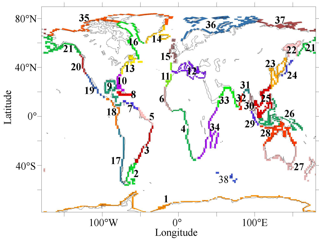
Figure 2. Model ^{228}\text{Ra} source regions
