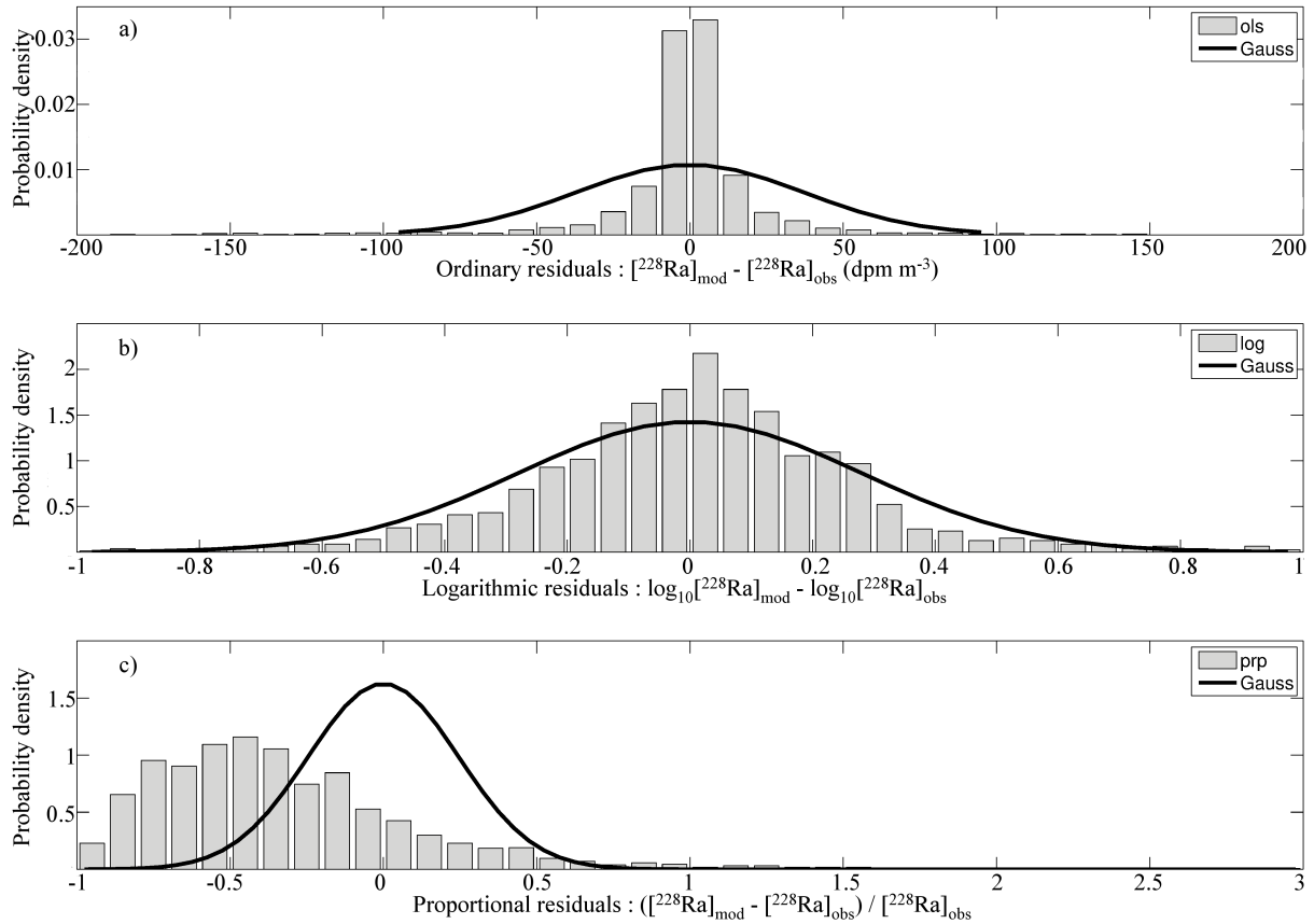
Figure 7. Probability Density Functions (PDF) of ^{228}\text{Ra} (a) ordinary residuals, (b) logarithmic residuals and (c) proportional residuals after inversion, compared with a Gaussian PDF (black full line) based on their standard deviations.
