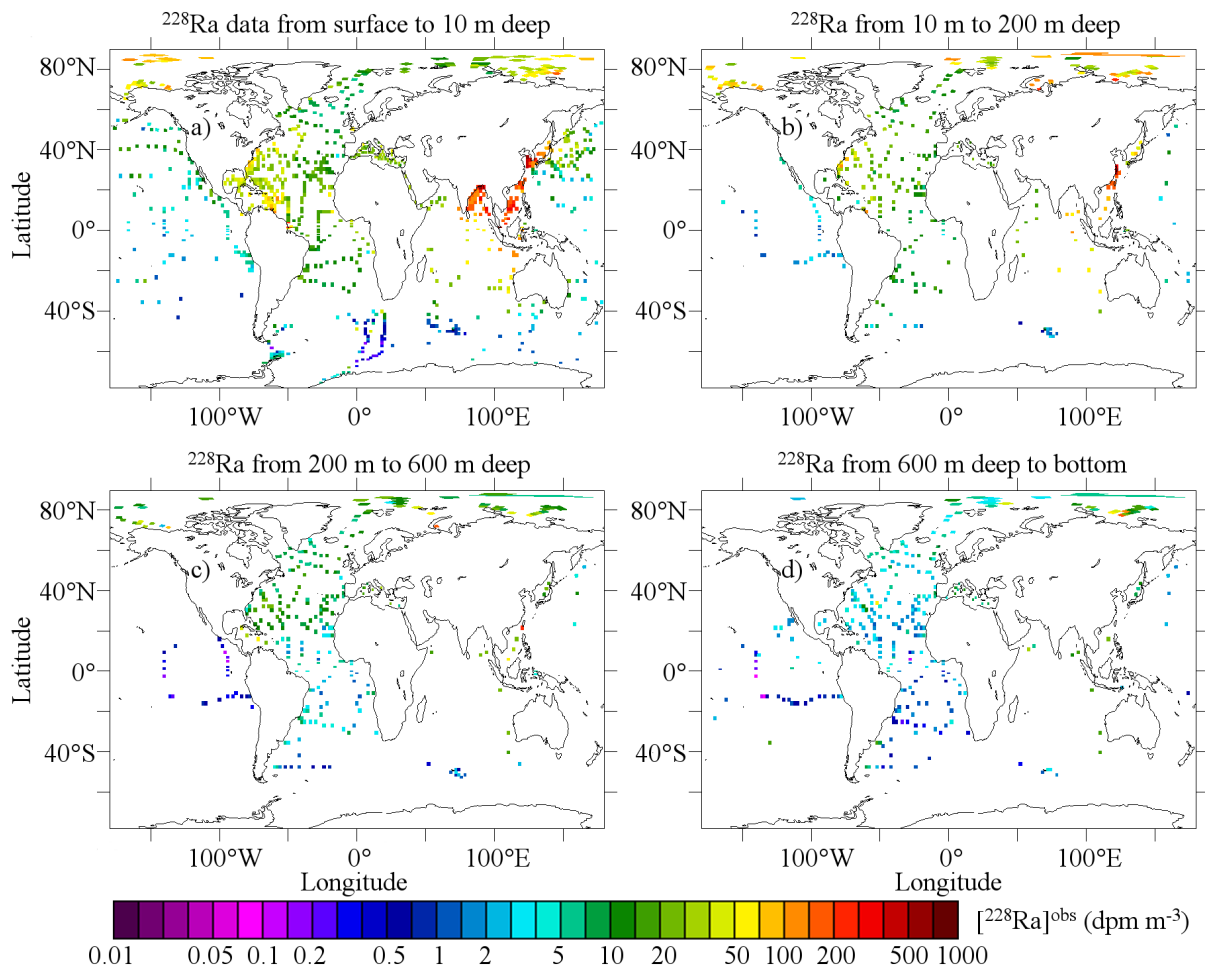
Figure 1. Observed concentrations of ^{228}\text{Ra} in the global ocean, averaged when available on the ORCA2 cells used for inversion. Data plotted on subfigures b), c) and d) are also vertically averaged in order to take all layers into account.
