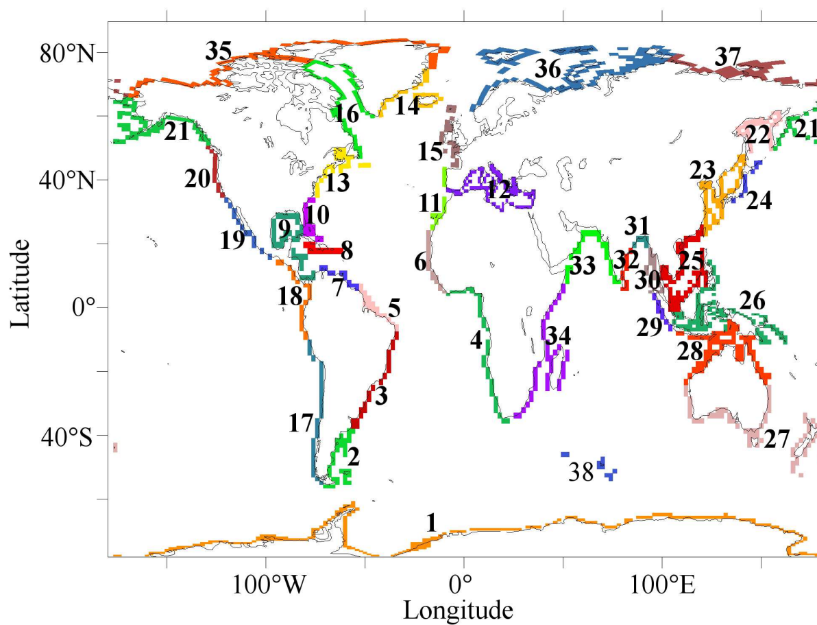
Figure 2. Model 228 Ra source regions
