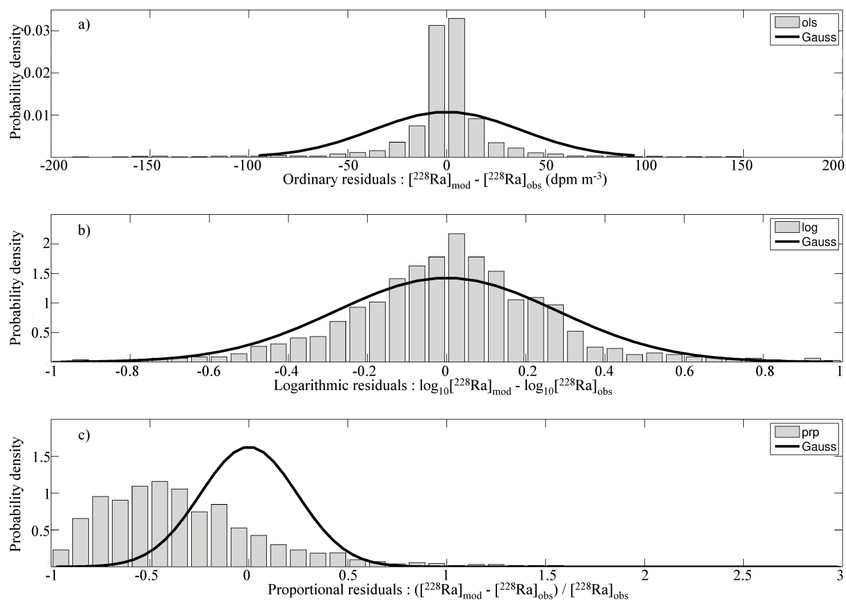
Figure 7. Probability Density Functions (PDF) of 228 Ra (a) ordinary residuals, (b) logarithmic residuals and (c) proportional residuals after inversion, compared with a Gaussian PDF (black full line) based on their standard deviations.
