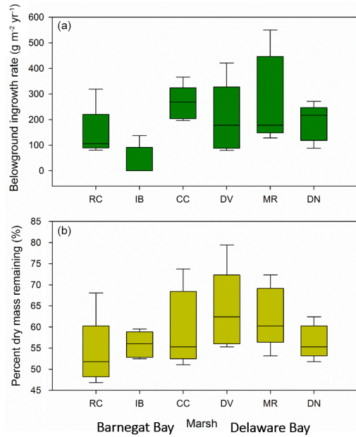
Figure 2. 137 Cs Belowground ingrowth rate (a) and percent mass remaining in belowground litterbags (b) over a 20-month period in salt marshes of two mid-Atlantic estuaries ( n = 5 , \pm standard error).
