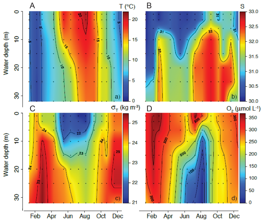
Fig. 1. Water column parameters (sampling station for this study at 23 m water depth). A: temperature [°C]. B: salinity. C: density anomaly [kg/m 3 ]. D: oxygen conc. [μmol/L]. From Hagens et al. (2015).
