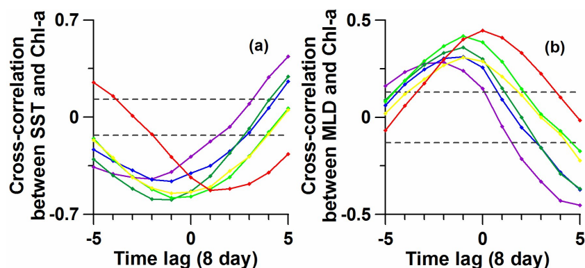
Figure 8. Cross-correlation of (a) SST and (b) MLD with Chl-a in six zones. Grey dashed horizontal line represents the 99 % confidence interval. Each tic on X-axis represents an 8-day period.
