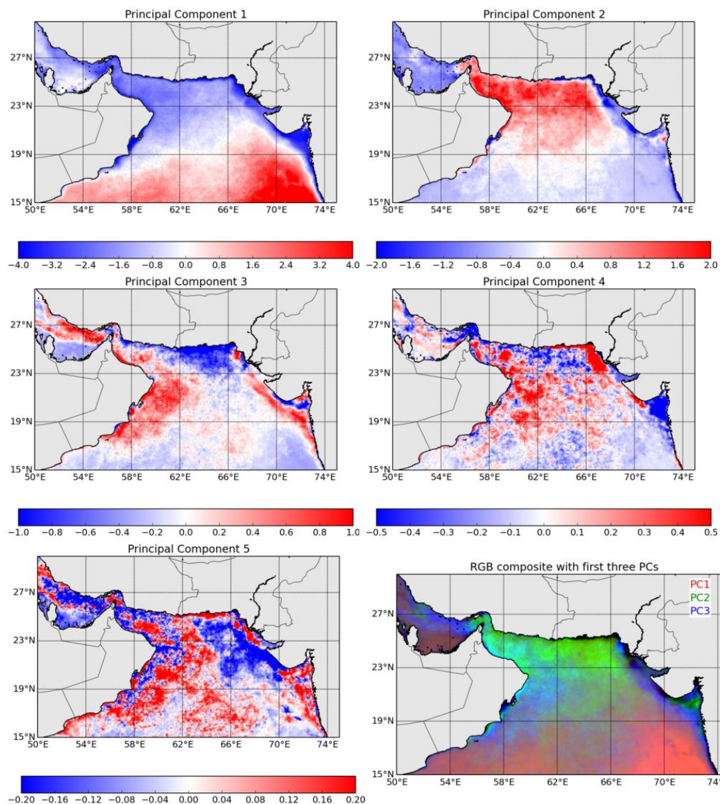
Figure 2. Individual maps of principal components (PC 1 to 5) and RGB composite of the first three statistically significant components.
