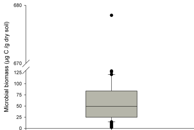
Figure 10. Boxplot of 206 observations of microbial biomass of soils under eucalyptus growing in southeast of Brazil (0-10 cm depth) (Prof. M. R. Tótolá pers. comm. )
