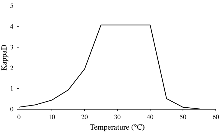
Figure 7. Effect of temperature on enzymatic kinetics represented by KappaD (Based on theoretical representation of Brock and Madigan, 1991).
