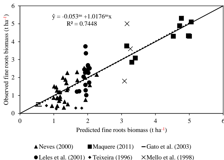
Figure 3. Observed fine root biomass (broke line) as a function of predicted values in relation to the 1:1 line (solid line). \beta_0 ( H_0=0 ) and \beta_1 ( H_0=1 ) were evaluated by t-test.
