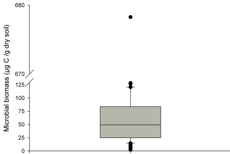
Figure 10. Boxplot of 206 observations of microbial biomass of soils under Eucalyptus growing in southeast Brazil (0-10 cm depth) (M. R. Tótoia pers. comm.)
