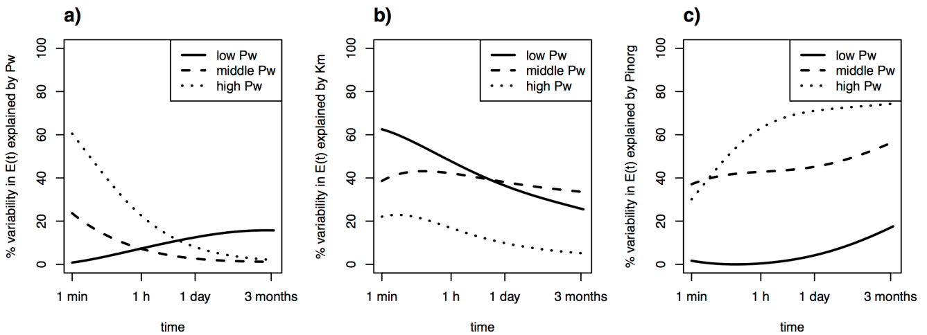
10 Figure 4: R^2 of simple linear regressions between isotopically exchangeable P ( E(t) ) explained by predictors P_w (a), K_m (b), and P_{inorg} (c) as a function of time. Regressions were fit separately for each class of P_w (low, middle, high), as determined by Jenks natural breaks optimization. Low P_w = 0.008 - 0.16 \text{ mg kg}^{-1} ( n = 46 ), middle P_w = 0.16 - 1.9 \text{ mg kg}^{-1} ( n = 94 ), and high P_w = 1.9 - 42.5 \text{ mg kg}^{-1} ( n = 77 ).
