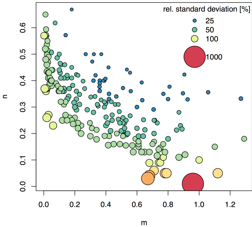
Figure 6: Relative standard deviations (RSD) of K_m after error propagation assuming 10% uncertainty in m and n input parameters, respectively. The plot shows the m and n values from the 217 soils included in this global compilation study. Uncertainty in K_m was approximated using the partial derivatives approach. Bubble size and color relates to the RSD of K_m for the plotted m and n combination.
