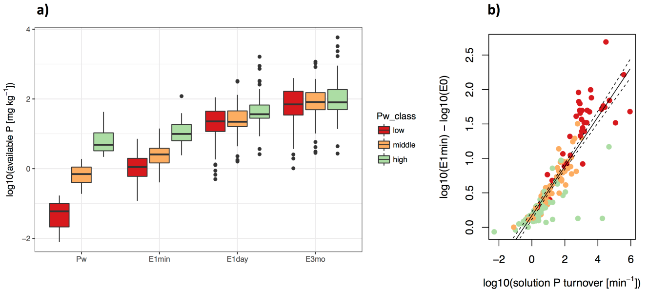
5 Figure 3: Soil solution P turnover ( K_m ) as a driver of available P ( E(t) ). While there is a large range in P availability at t = 0 ( P_w ), this variability becomes smaller and gradually uncoupled from P_w class for longer time frames ( t=1, 1440, 129'600 min) (a). The growth in P availability between t=0 and t = 1 is dependent on K_m (b). Simple linear regression between K_m and the difference between E(t) and E(0) is given by \log_{10}(E(1)) - \log_{10}(E(0)) = 0.170 + 0.357 * \log_{10}(K_m) with F = 615 , p < 10^{-15} , and R^2 = 0.79 . n = 170 . Red, orange, and green colors refer to low, middle, and high P_w -classes as determined by Jenks natural breaks optimization. In (b), dashed lines represent the 95% confidence interval.
