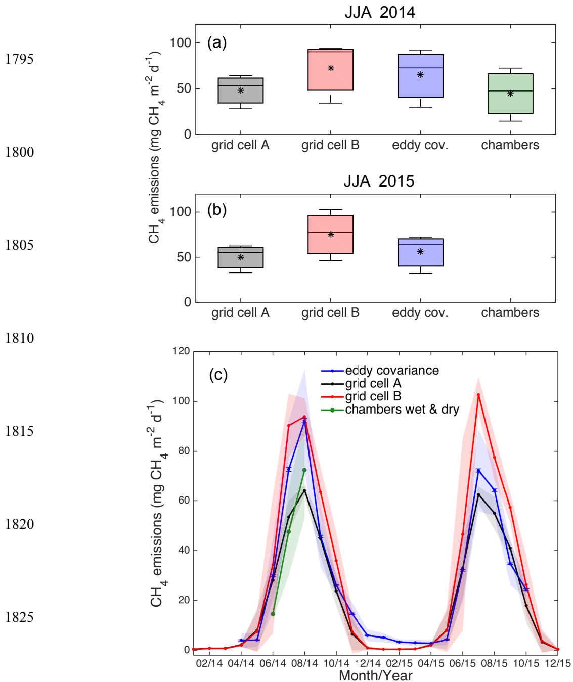
1830 Figure 5 – Box plot for summer (JJA) methane emissions from model grid cells A and B, eddy covariance and chamber flux measurements for a) 2014 and b) 2015 (without chamber flux measurements). The central horizontal line on each box is the median for each data set and whiskers are the minimum and maximum values; c) time series of monthly CH 4 emissions for 2014 and 2015 for grid cells A and B in the model, from eddy covariance as well as chamber flux measurements. Shaded areas depict one standard deviation of the monthly mean of each data set calculated from the daily resolution model output. Error bars in the EC fluxes are the uncertainty of the monthly averages of the gapfilled and quality checked signal.
