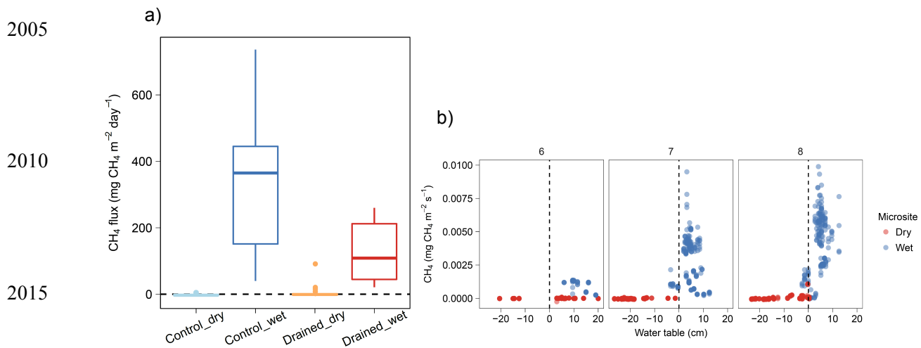
Figure A3 - Daily methane flux rates a) aggregated from flux chamber measurements within the growing season of 2014. Measurements are separated into drained (1 wet microsite, 9 dry microsites) and control (8 wet microsites, 2 dry microsites) transects; b) flux rates against the water table at each microsite. Dry plots had a water table at or below the surface (up to 10 cm), whereas wet plots had a water table at or above the surface.
