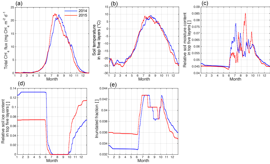
1945 Figure 10 – Mean daily ancillary variables and CH 4 emissions in the model domain in 2014 and 2015: a) total CH 4 emissions, b) mean soil temperature in the root zone (top five soil layers), c) domain mean relative soil moisture content in the top five soil layers, d) domain mean relative soil ice content in the top five soil layers, e) inundated fraction of the grid cell
