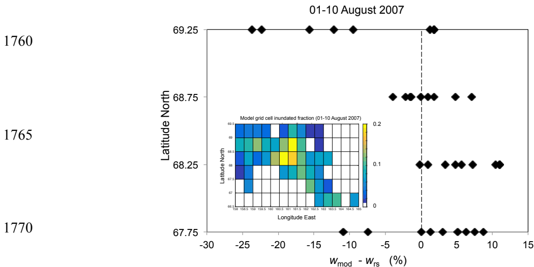
1760 1765 1770 1775 Figure 2 – Latitudinal distribution of the difference between the fractions of the grid cell inundated areas simulated with TOPMODEL in JSBACH-methane ( w_{mod} ) and the inundated areas estimated from the EAWS product ( w_{rs} ) for the same grid cells (01-10 August 2007). Inset figure is the mean spatial distribution of the fraction of inundated areas in the model domain for 01-10 August 2007. Grid cells with inundated areas < 1 % are not shown.
