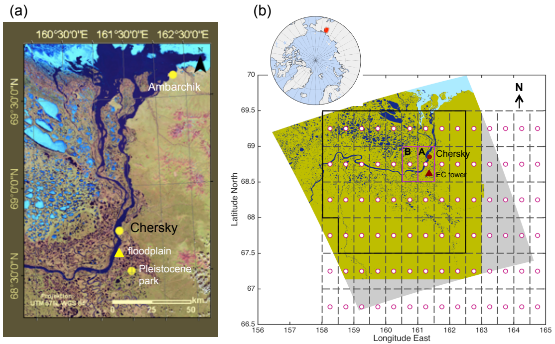
1750 Figure 1 – a) MODIS image showing the heterogeneous landscape in most of the model domain in Northeast Siberia, also showing the location of nearby cities and the floodplain, b) geographical location of the model domain used in this study also depicted with the midpoints of the model grid cells (pink circles) and boundaries (dashed lines) underlain by a geoTIFF image (data from 01-10 July 2007) from the EAWS product. The boundaries of the grid cells A and B are delimited with pink lines. The continuous dark line delimits the 35 model grid cells used for the evaluation of modeled inundated areas against the EAWS product.
