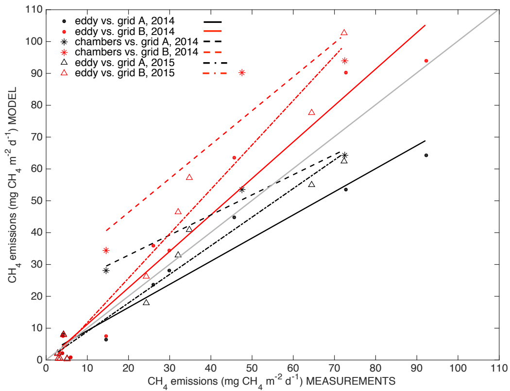
1790 Figure 4 – Comparison between modeled CH 4 emissions and flux measurements by chambers and EC in the Chersky floodplain: correlation between results for model grid cells A and B and measurements during 2014 and 2015 (the light grey line is the 1:1 line).
