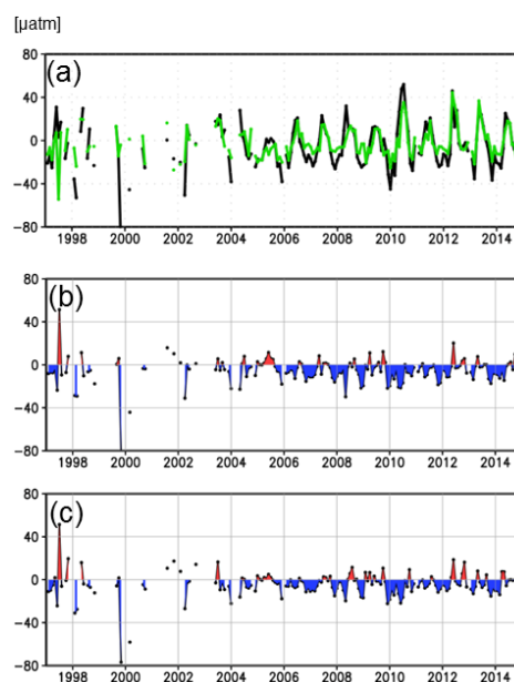
Figure A: (a) pCO 2 bias (estimate – observation) averaged over the entire analysis area [μatm], for the estimates with Chl-a (green) and without Chl-a (black). Difference in (b) absolute bias and (c) RMSD for pCO 2 estimated with and without Chl-a averaged over the entire analysis area [μatm]. Negative value means improvement of the estimates in b and c.
