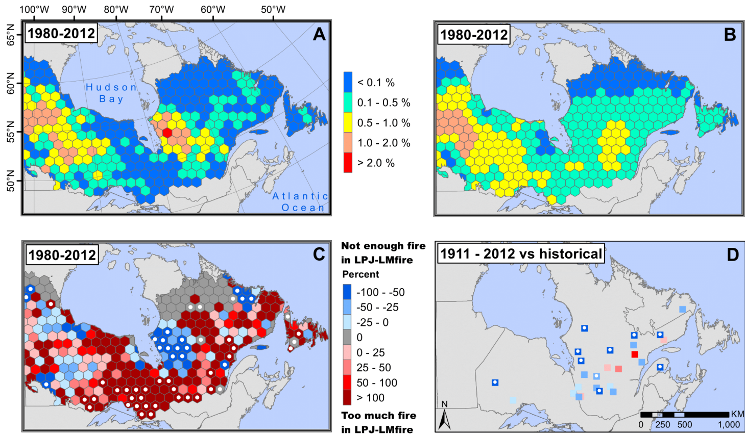
5 Figure 2. Observed versus LPJ-LMfire-simulated annual burn rates across eastern boreal Canada. (A) Observed annual burn rates computed for 365 hexagonal cells between 1980 and 2012 (data from Natural Resources Canada, 2017). (B) LPJ-LMfire simulated annual burn rates computed over the same period and hexagonal cells. (C) Percent age of difference between observed and simulated annual burn rates. (D) Percent age of difference between historical annual burn rates reconstructed from stand-replacing fire history studies (data from Girardin et al., 2013b; Héon et al., 2014; Portier et al., 2016) and LPJ-LMfire-simulated annual burn rates between 1911 and 2012 (see Supplement S4 for further details). White points indicate where the observed (and historical) annual burn rate lies outside the 95% confidence interval (95% CI) of the averaged annual burn rates in hexagonal cells simulated by LPJ-LMfire.
