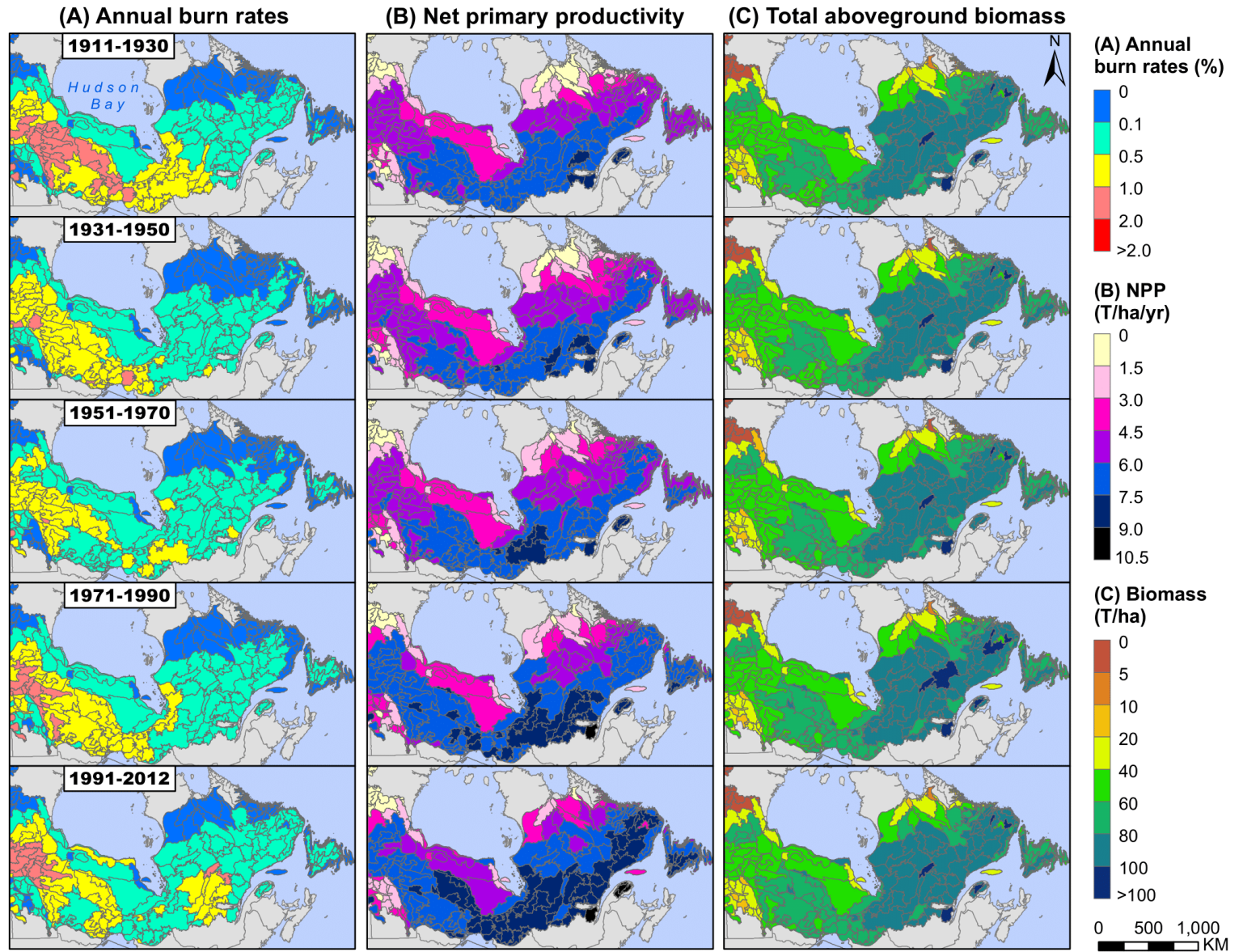
Figure 5. LPJ-LMfire simulated (A) annual burn rates (%), (B) net primary productivity (T/ha/yr) and (C) total aboveground biomass (T/ha) across eastern boreal Canada for five periods between 1911 and 2012.
