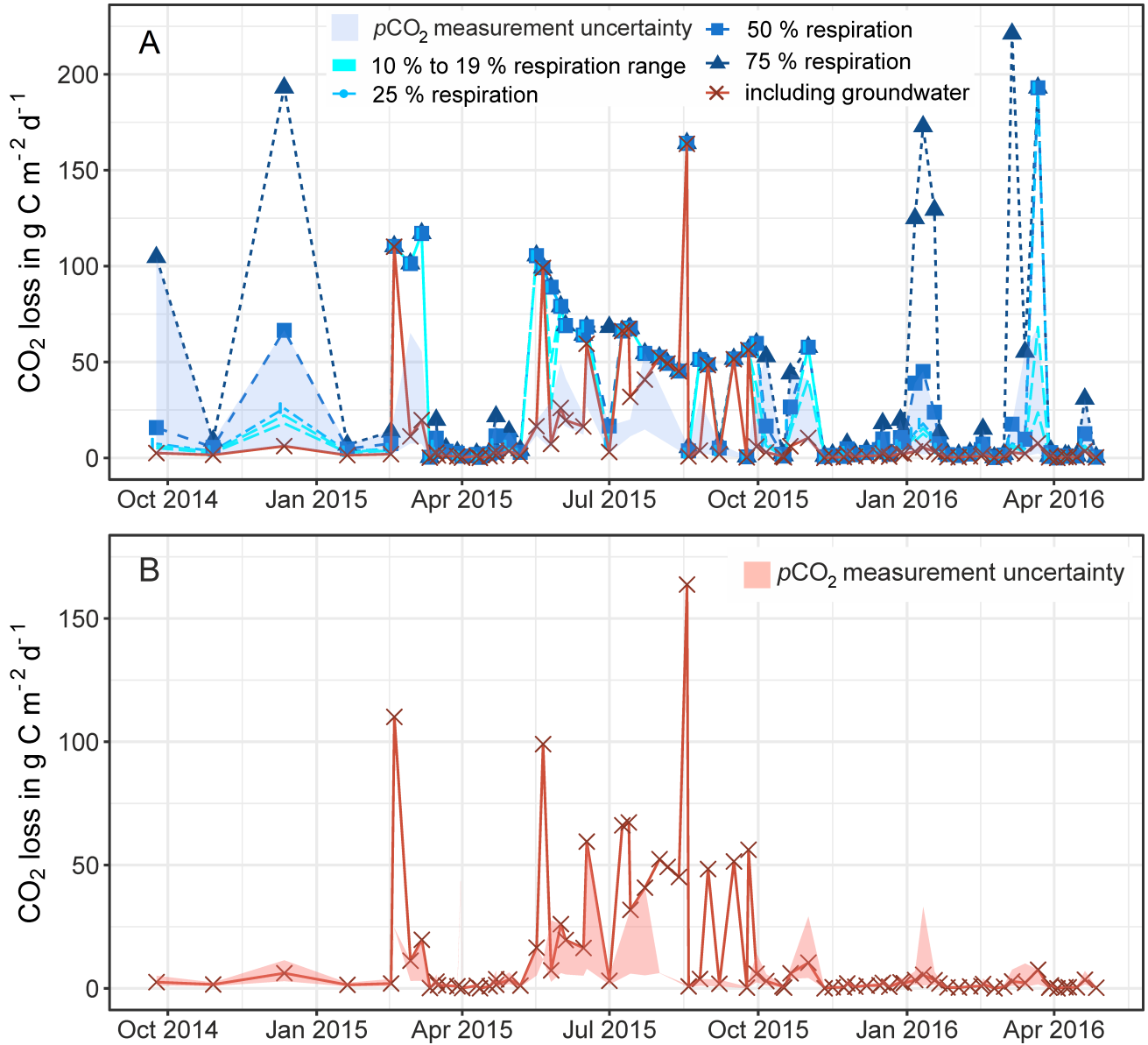
5 Figure 3: Modelled carbon dioxide loss via outgassing from the stream to the atmosphere upstream of the Uhlirska catchment outlet (UHL) based on the model by Polsenaeere and Abril (2012) for proportion river respiration ( R ) between 10 and 75 % (A) and modified with measured groundwater \delta^{13}C_{DIC} (A and B). The areas shaded in blue (A) and red (B) indicate uncertainties in calculation of pCO_2 with \pm 21 %. Convergence criteria were not fulfilled for data points that lie outside the shaded area (see section 3.1).
