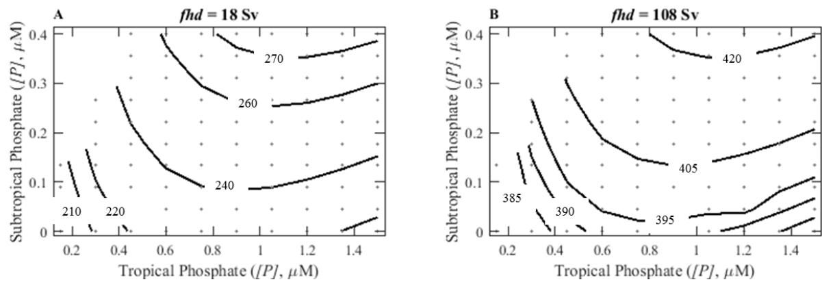
Figure 2: pCO_{2,atm} (ppm) sensitivity to extreme fhd values under changing surface phosphate concentrations. A.) Range of pCO_{2,atm} (ppm) using an fhd value of 18 Sv. B.) Range of pCO_{2,atm} (ppm) using an fhd value of 108 Sv.
