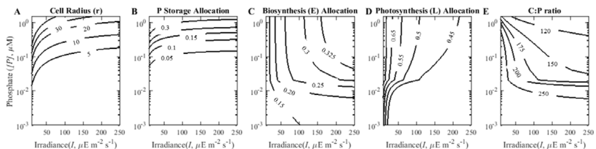
Figure 5: Influence of phosphate concentration and irradiance on cellular stoichiometry and cellular traits, at a constant T = 25\text{ °C} . A) Cell radius ( r ). B) P storage allocation. C) Biosynthesis allocation. D) Photosynthesis ( L ) allocation. E) The C:P ratio. As irradiance increases, there is a tendency towards greater allocation to biosynthesis and lesser allocation to photosynthesis, which leads to lower C:P ratios. When phosphorus is very low, there is a large decrease in both biosynthesis and photosynthesis allocations due to the large relative allocation to the cell membrane. C:P ratios are inversely proportional to phosphorus concentration, driven by an increase in luxury storage and ribosomal content as P increases.
