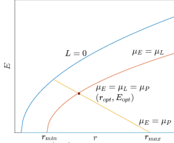
Figure 4: Diagram of strategy space. The (r, E) plane is divided into a region in the first quadrant where L > 0 , corresponding to the set of allowable strategies. The optimal strategy occurs at the point (r_{opt}, E_{opt}) , denoted by the red rectangle, where \mu = \mu_L = \mu_P = \mu_E .
