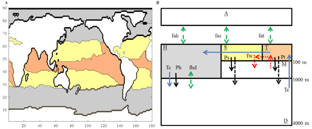
Figure 1: Box Model Design. A) Sea surface breakdown by region. All peach-colored regions represent the tropical surface ocean box, the cream-colored regions represent the subtropical surface ocean box, and grey regions represent the high-latitude surface ocean box. B) The model includes tropical ( T ), subtropical ( S ), and high-latitude ( H ) surface ocean boxes, a mixed thermocline ( M ) box, and a deep water ( D ) box. The thermohaline circulation T_c is set to 20 Sv, while the wind driven shallow overturning circulation is set to 5 Sv. The high-latitude mixing flux f_{hd} is set to 45.6 Sv. The thickness of Box H is 1000 m, and Box M is 900 m. Box T has a temperature of 26°C, box S has a temperature of 24°C, and box H has a temperature of 7°C. Box S covers 39% and Box T covers 25% of the ocean surface area.
