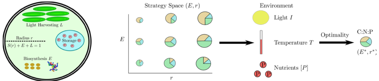
Figure 3: Diagram of physiological model. Phytoplankton strategies are represented in a two-dimensional strategy space ( E, r ). Each strategy is assigned a fitness in each environment using physiological principles, and the strategy with the highest fitness is selected to represent the local population. The stoichiometry of cellular components is used to calculate the stoichiometry of the functional pools in the cell.
