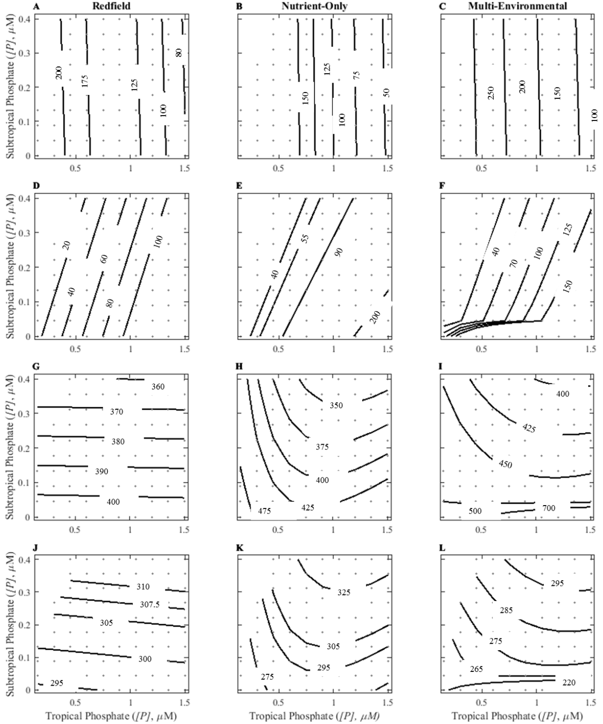
Figure 9: Carbon export ( \text{Tmol C yr}^{-1} ) and p\text{CO}_{2,\text{atm}} (ppm) in changing surface phosphate concentrations. Columns correspond to type of stoichiometry; Redfield (Left), nutrient-only (Middle), and multi-environmental model (Right). Rows correspond to either tropical carbon export (A through C), subtropical carbon export (D through F), total carbon export (G through I) or atmospheric p\text{CO}_2 (J through L). The grey points represent where p\text{CO}_{2,\text{atm}} was calculated, between spaces are interpolated.
