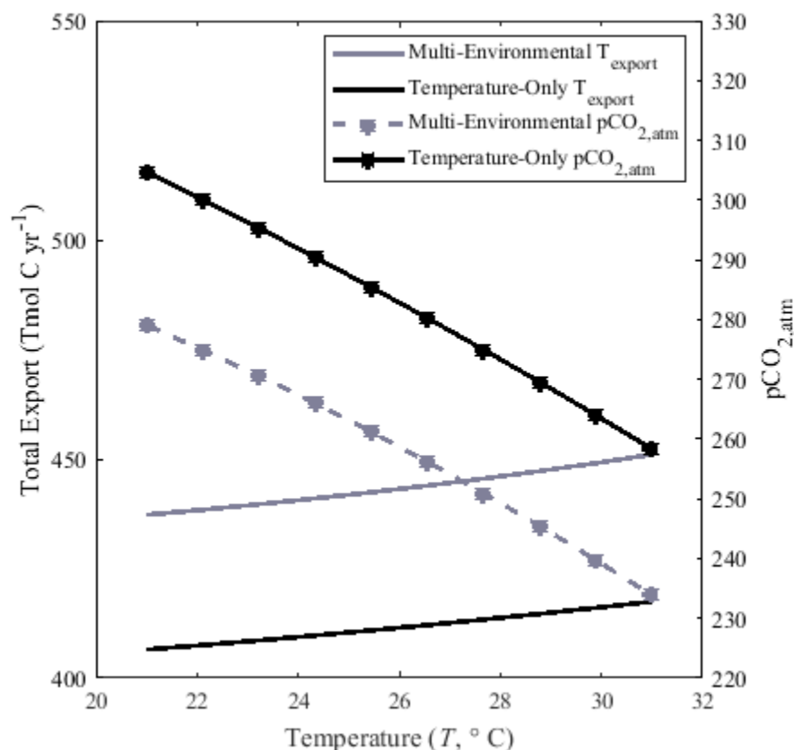
705 Figure 11: The effect of changing sea surface temperature (°C) on p\text{CO}_{2,\text{atm}} and total carbon export (Tmol \text{C yr}^{-1} ) in the temperature-only and multi-environmental model. Phosphate concentrations are 0.3 \mu\text{M} in the tropical and 0.05 \mu\text{M} in the subtropical box. Multi-environmental model total carbon export is the solid gray line, and p\text{CO}_{2,\text{atm}} is the dashed gray line. Temperature-only model total carbon export is the solid black line, and p\text{CO}_{2,\text{atm}} is the dashed black line.
