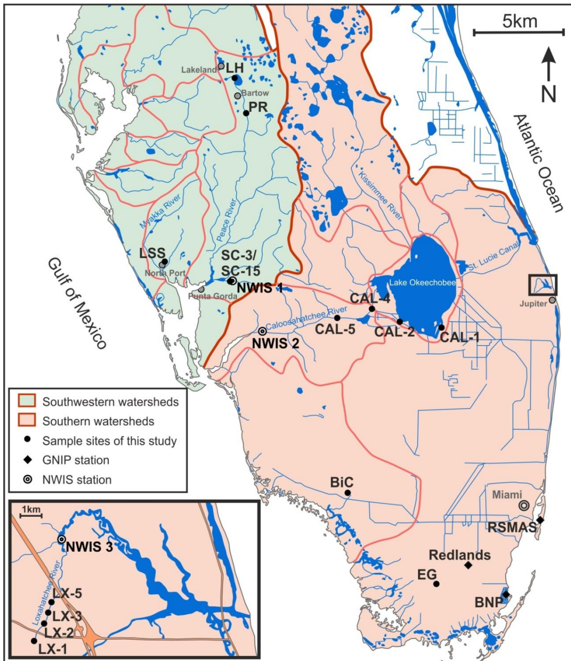
Figure 2: Location of sample sites (BiC=Big Cypress Swamp, CAL=Caloosahatchee River, EG=Everglades, LH= Lake Hancock, LSS=Little Salt Spring, LX= Loxahatchee River, PR= Peace River, SC=Shell Creek). Also included are GNIP stations (Redlands, RSMAS, BNP) and NWIS stations (NWIS 1=02297635; NWIS 2=02292900; NWIS 3=265906080093500).
