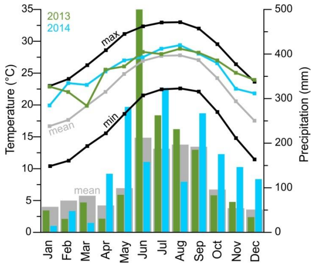
Figure 1: Fifty-years average (1955-2005) of maximum and minimum temperatures and mean precipitation of the southwestern and southern catchment area of Florida in comparison to mean temperature and mean precipitation of Miami 2013 (green) and 2014(blue) (National Climate Change Viewer, U.S. Geological Survey; http://www2.usgs.gov/climate_landuse/clu_rd/nccv.asp ; Adler and Hostetler, 2013).
