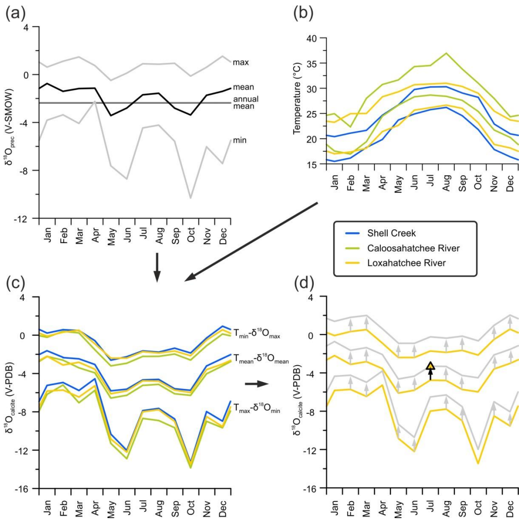
Figure 3: Modelling of the monthly composition of a theoretical calcite formed in equilibrium in Florida rivers (a) precipitation \delta^{18}\text{O} ; (b) water temperature from rivers in Florida; (c) calculated calcite ranges using equation (1); (d) example for the offset correction from LX-4. For detailed explanations see text (chapter 3.4).
