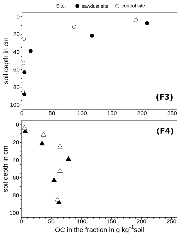
Figure 5. Organic carbon concentrations of fraction three and four related to the bulk soil mass. These fractions comprise organic matter strongly bound to mineral phases in soil particles of densities between 1.6-2.0 (F3) or >2.0 g cm -3 (F4).
