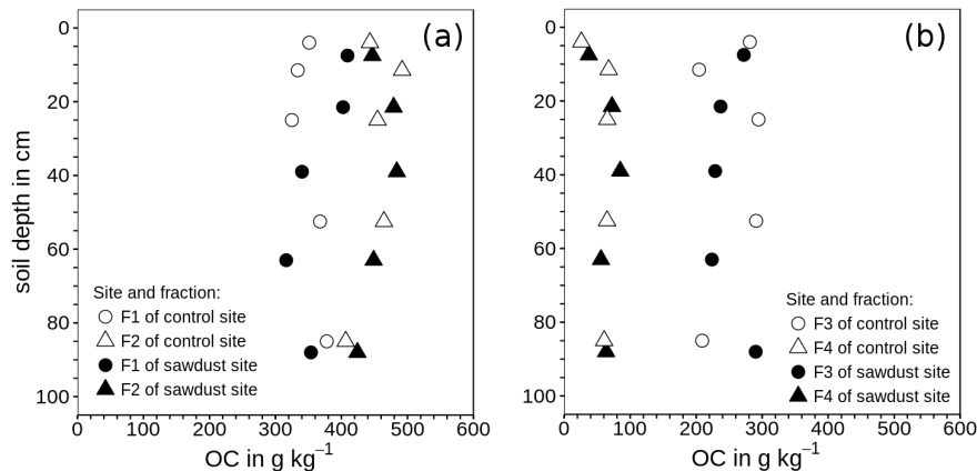
Figure 3. Mean of organic carbon (OC) concentrations in density fractions one to four related to the mass of the respective fraction instead of the bulk soil mass. (a) Fractions 1 (F1) contains material released directly; fraction 2 (F2) represents material released after applying 300 J ml -1 sonication energy. (b) Fractions 3 and 4 comprise organic matter strongly bound to mineral phases in soil particles of densities between 1.6-2.0 (F3) and >2.0 g cm -3 (F4).
