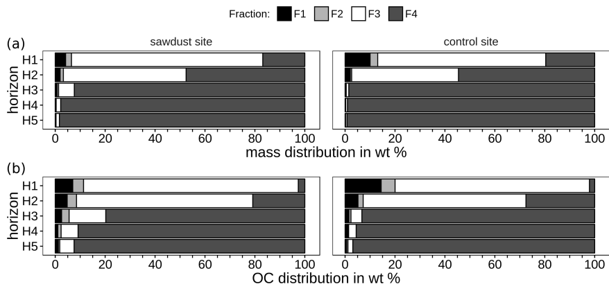
Figure 4. Mass (a) and organic carbon (OC, b) distribution over density fractions, given as percentages of cumulated fractions. Fraction 1 and 2 contain material either, directly released (F1) or after applying 300 \text{ J ml}^{-1} sonication energy (F2). Fractions 3 and 4 comprise organic matter strongly bound to mineral phases in soil particles of densities between 1.6\text{-}2.0 \text{ g cm}^{-3} (F3) or >2.0 \text{ g cm}^{-3} (F4).
