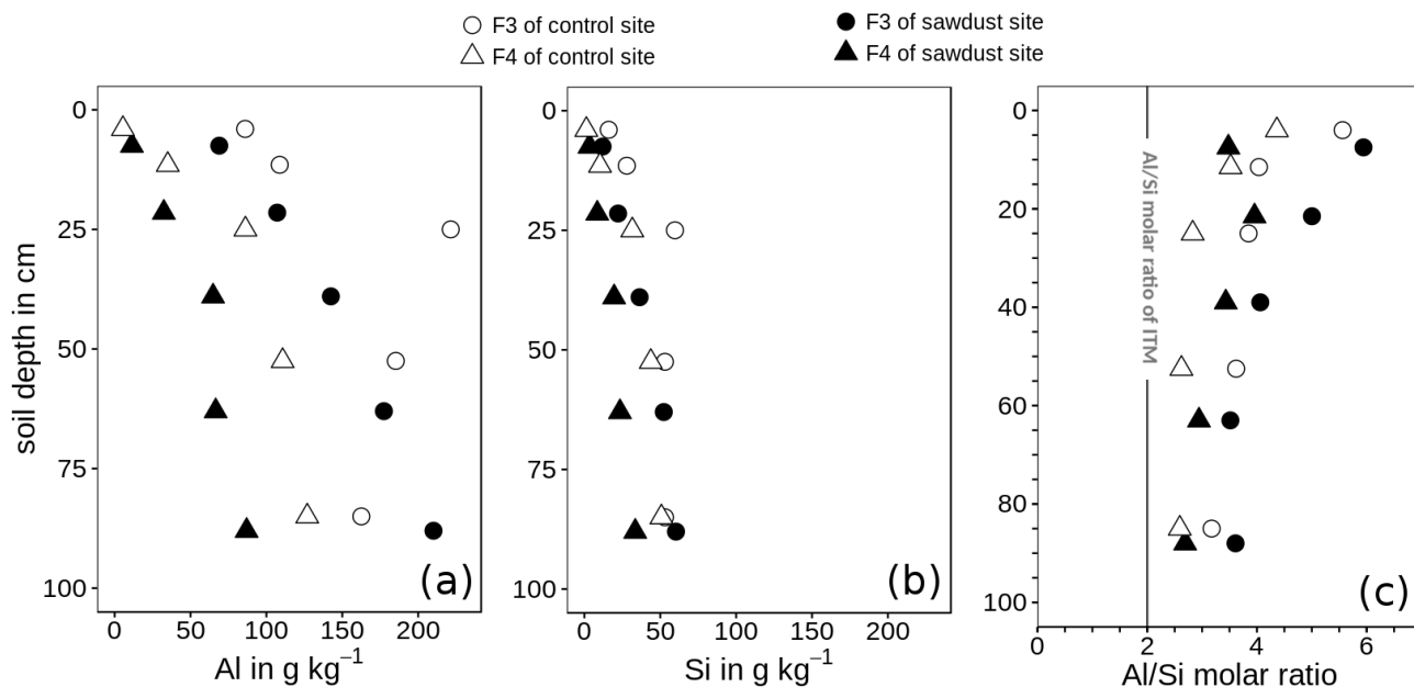
Figure 6. Concentration of acid oxalate-extractable aluminium (Al, a) and silica (Si, b) and Al/Si molar ratios (Al/Si, c) of fractions of densities between 1.6-2.0 (F3) and >2.0 \text{ g cm}^{-3} (F4). The metal concentrations are normalized to the mineral portion of the fraction, assuming that the mass of OM is two times the mass of OC (Sollins et al., 2006). ITM: imogolite-type mineral phases.
