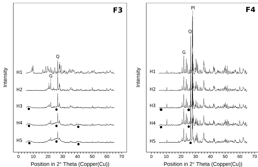
Figure 7. X-ray diffractograms (Cu-K \alpha radiation) of the heavy fractions for all horizons of samples from the sawdust site. Fraction 3 and 4 comprise particles of densities between 1.6-2.0 (F3) and >2.0 \text{ g cm}^{-3} (F4). All diffractograms are normalized to the same vertical scale. Circles indicate poorly crystalline material. Q marks the main quartz reflex. PI marks the main plagioclase reflex. G marks the main gibbsite reflex.
