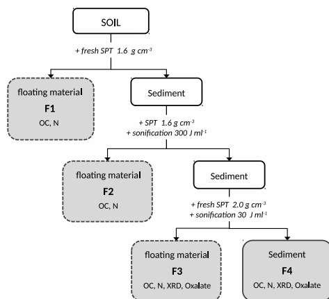
Figure 1. Sequential density fractionation scheme. SPT: sodium-polytungstate solution, F1: fraction predominately organic matter of densities <1.6 \text{ g cm}^{-3} , with basically no interaction with the mineral phase, F2: fraction predominately organic matter of densities <1.6 \text{ g cm}^{-3} and weakly associated with the mineral phase, F3: soil materials of densities between 1.6 and 2.0 \text{ g cm}^{-3} and holding organic matter strongly bound to mineral phases, F4: soil materials of densities >2.0 \text{ g cm}^{-3} and holding organic matter strongly bound to mineral phases. Below the fraction labeling subsequent analyses are listed. OC: total organic carbon concentration, N: nitrogen concentration, XRD: X-ray diffraction, Oxalate: ammonium oxalate-oxalic acid extraction
